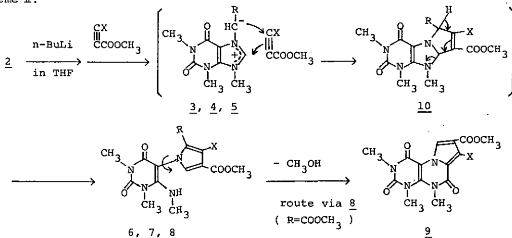
Scheme II.
