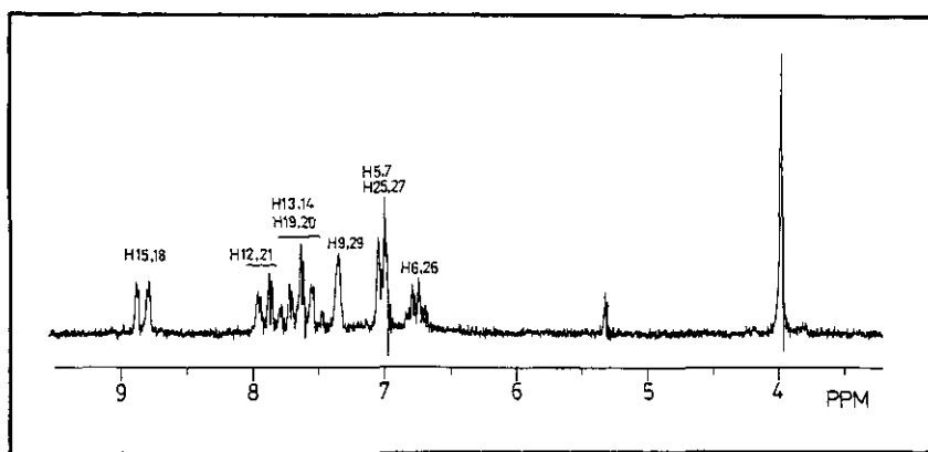
FIGURE 1 1 H NMR spectrum of 6 determined in CD 2 Cl 2 at 35°C on a Perkin Elmer R32 (90 MHz) spectrometer.
