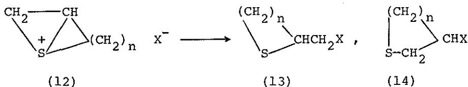
Scheme I
