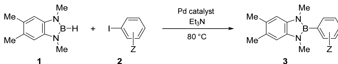
Scheme 1. Borylation of aryl iodides 2 with 2,3-dihydro-1 H -benzo[ d ][1,3,2]diazaboroles 1
