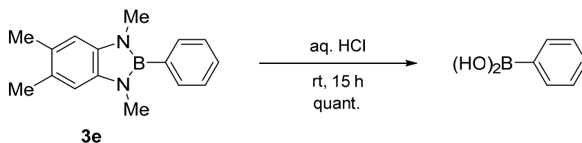
Scheme 2. Deprotection of 3e to phenylboronic acid
