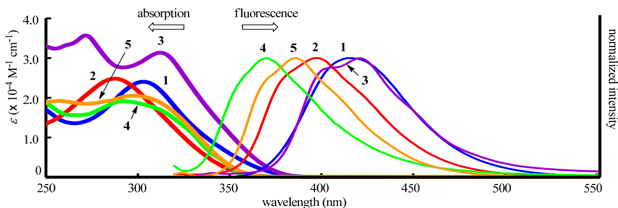
Figure 1. UV-VIS absorption (bold line; 3.0 \times 10^{-5} M in THF) and fluorescence (narrow line; 3.0 \times 10^{-7} M in THF, excited at \lambda_{\text{max}} ) spectra of 1 (blue line), 2 (red line), 3 (purple line), 4 (green line), and 5 (orange line)
