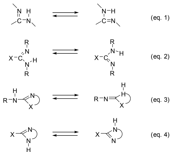
Figure 3. Tautomeric equilibria
