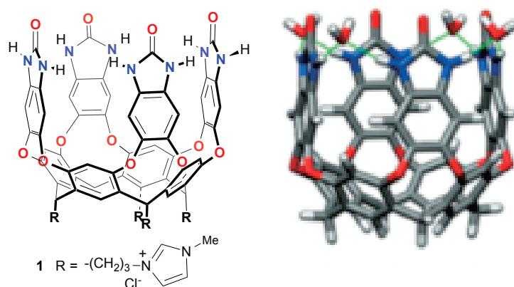
Figure 1. Left, chemical formula of the water-soluble, deep cavitaand 1 . Right, a modeled structure of the vase-like form; the 4 water molecules stabilize the vase conformation through hydrogen bonding. The “feet” have been truncated.
