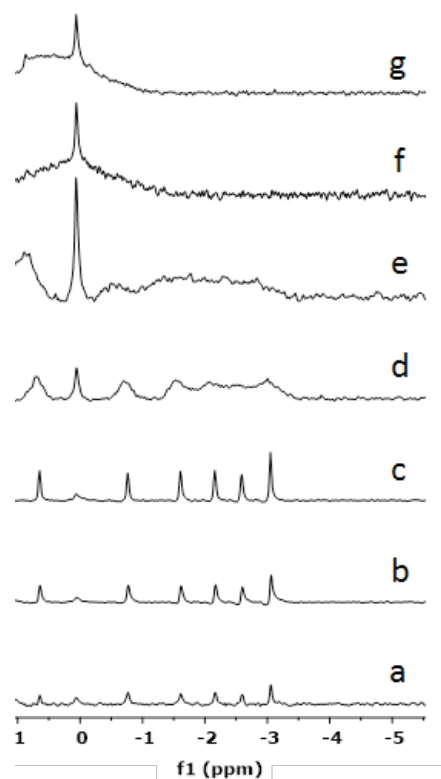
Figure 3. Partial ^1\text{H} NMR (600 MHz, \text{D}_2\text{O} , 298 K) spectra of the complexes of 1 (1.0 mM) with sub-stoichiometric amounts and excess of 2-nonenal 2 ; The upfield shifts of the \text{CH}_2 and \text{CH}_3 groups place them deep in the cavity of 1 . Spectra after addition of (a) 0.05 equiv., (b) 0.2 equiv., (c) 0.6 equiv., (d) 0.85 equiv., (e) 1.1 equiv., (f) 1.6 equiv., (g) 2.0 equiv. of aldehyde.
