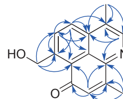
Figure 2. Key HMBC (↷) correlations of 1
