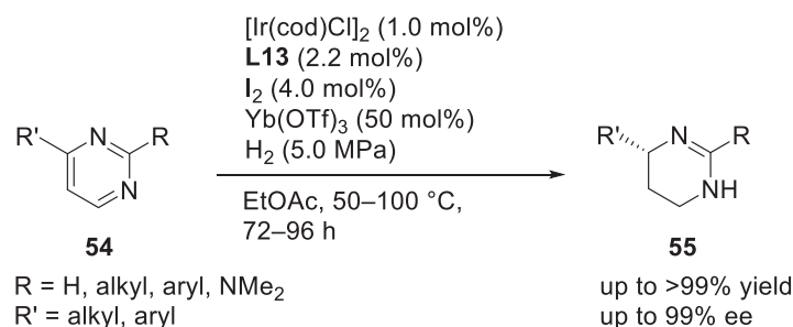
Scheme 20. Asymmetric Hydrogenation of Pyrimidines 54 Catalyzed by Iridium(I) Complex
