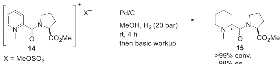
Scheme 7. Asymmetric Hydrogenation of N -Methylated Pyridinium Salt 14
