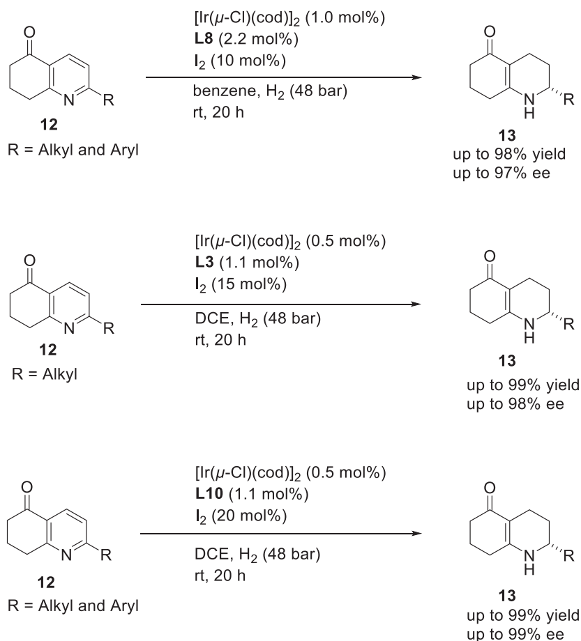
Scheme 6. Asymmetric Hydrogenation of 12
