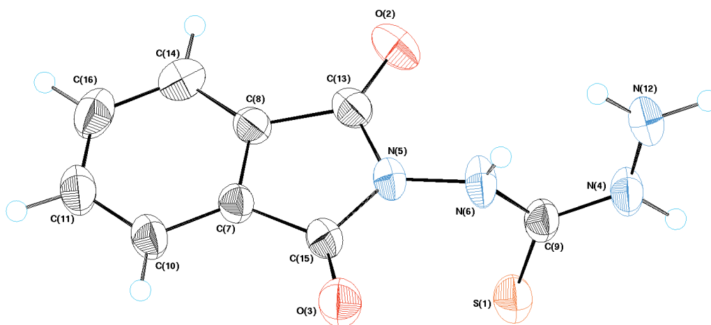
Figure 1. X-Ray structure of 4
