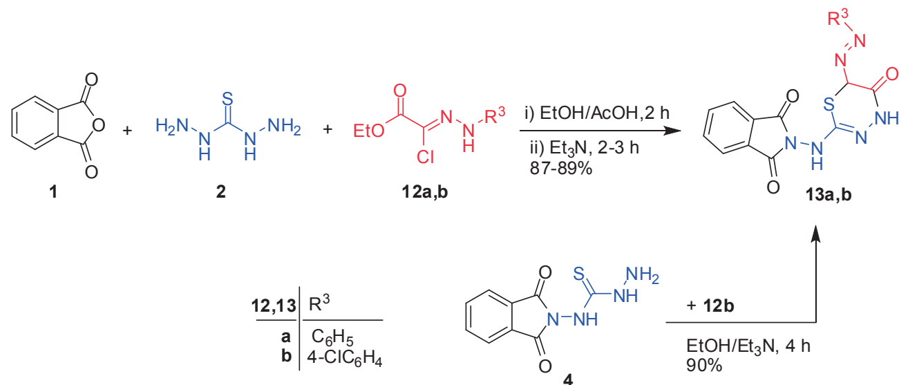
Scheme 4
