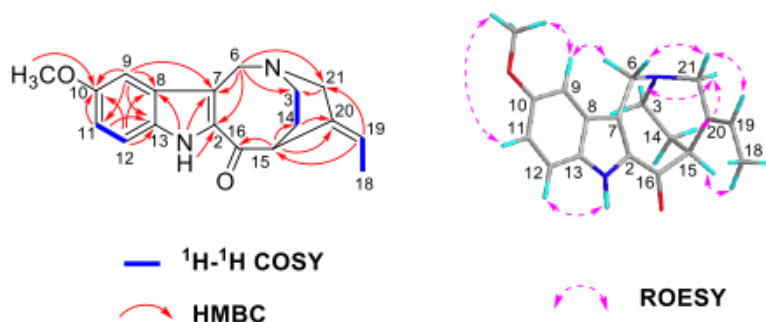
Figure 2. Selected 2D NMR correlations for 10-methoxyconolidine ( 1 )
