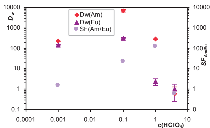
Figure 4. Extraction of Am(III) and Eu(III) by CyMe 4 -BTPhen-functionalized SiO 2 gel 8 as a function of HClO 4 concentration. Mass of sorbent: approximately 15 mg, phase volume: 0.6 mL, V/m ratio: \sim 40 mL g -1
