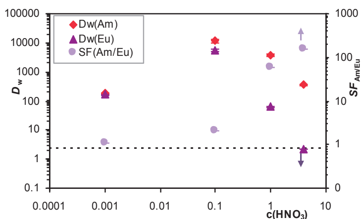
Figure 3. Extraction of Am(III) and Eu(III) by CyMe 4 -BTPhen-functionalized SiO 2 gel 8 as a function of HNO 3 concentration. Mass of sorbent: approximately 16 mg, phase volume: 1 mL, V/m ratio: \sim 60 mL g -1
