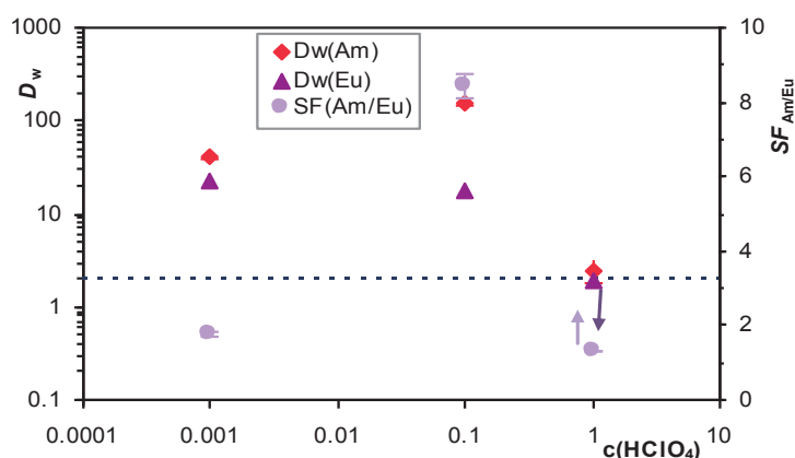
Figure 5. Extraction of Am(III) and Eu(III) by CyMe 4 -BTPhen-functionalized SiO 2 -coated MNPs 4 as a function of HClO 4 concentration. Mass of sorbent: approximately 18 mg, phase volume: 0.6 mL, V/m ratio: ~ 33 mL g -1
