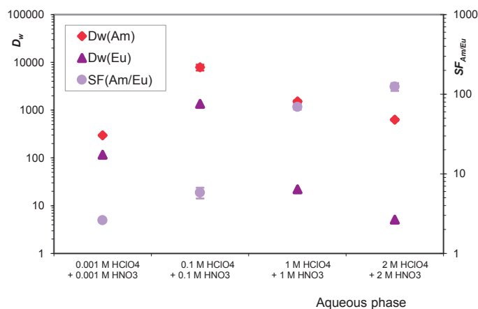
Figure 6. Extraction of Am(III) and Eu(III) by CyMe 4 -BTPhen-functionalized SiO 2 gel 8 as a function of HClO 4 / HNO 3 concentration. Mass of sorbent: approximately 15 mg, phase volume: 0.6 mL, V/m ratio: ~ 40 mL g -1
