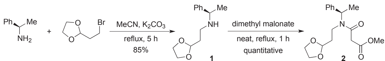
Scheme 2. Synthesis of chiral malonylamide intermediate 2
