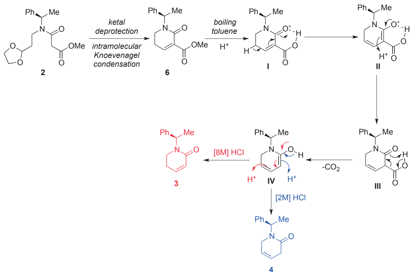
Scheme 5. Plausible mechanism for regioselective formation of compounds 3 and 4
