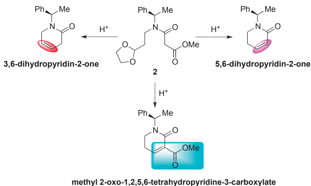
Scheme 1. Divergent synthesis of 3,6- and 5,6-dihydropyridin-2(1 H )-ones via intramolecular Knoevenagel condensation
