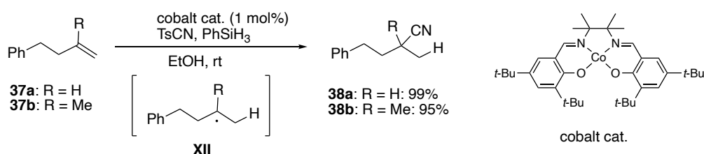
Scheme 24. Carreira's Hydrocyanation Using Simple Olefins Under Co catalysis
