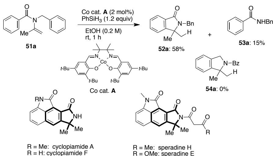
Scheme 31. Initial Attempt for Hydroarylation
