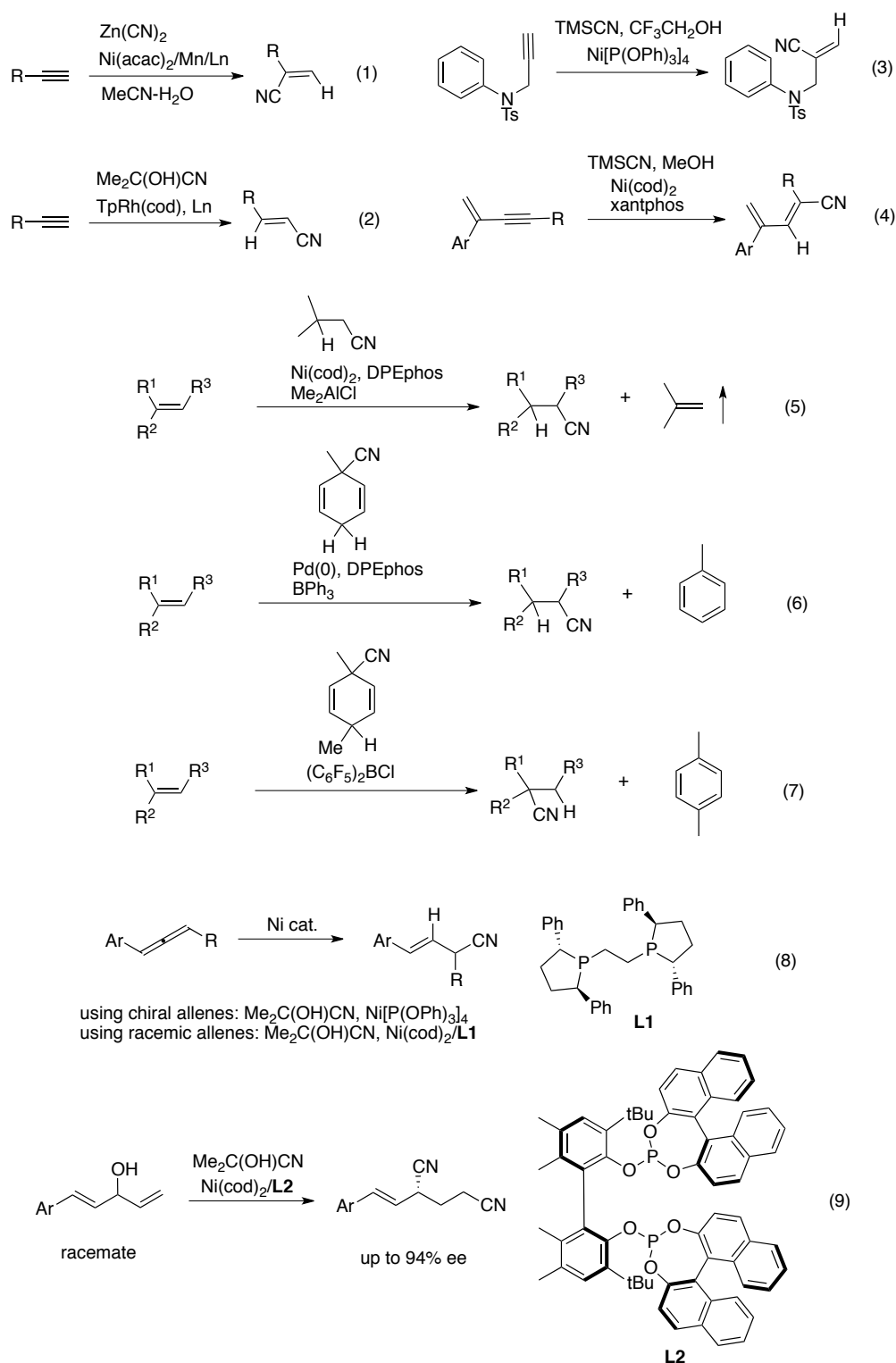
Scheme 16. Recent Hydrocyanation Under Metal Catalysis
