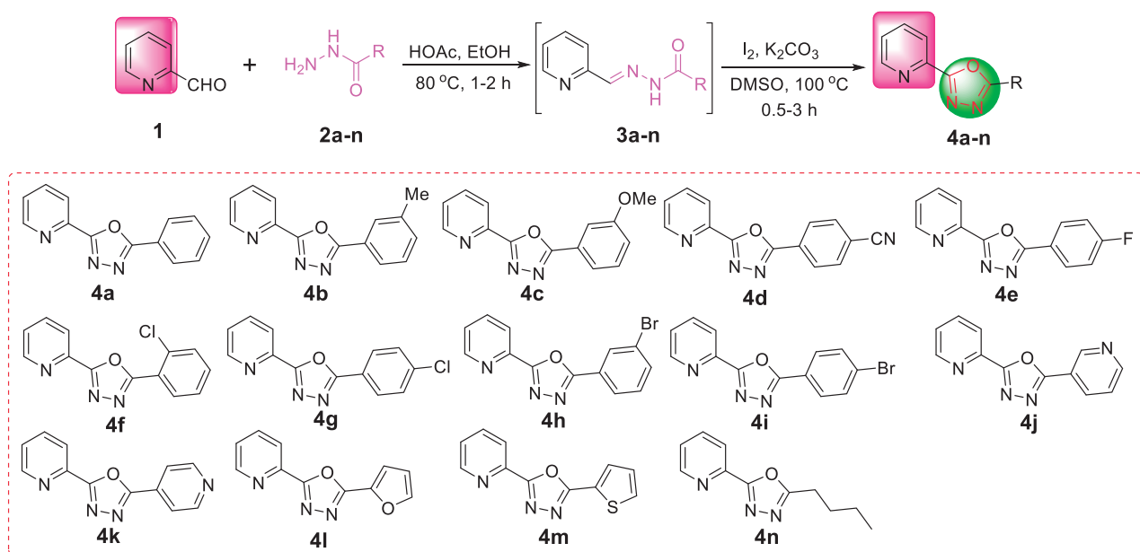
Figure 1. Synthetic route and chemical structure of pyridine-based 1,3,4-oxadiazole derivatives ( 4a-n )
