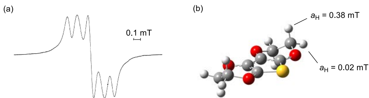
Figure 6. (a) ESR spectrum of 4 with \text{SbCl}_5 in \text{CH}_2\text{Cl}_2 at room temperature. (b) Optimized structure of \mathbf{4}^{+\bullet} with calculated hyperfine coupling constants.
