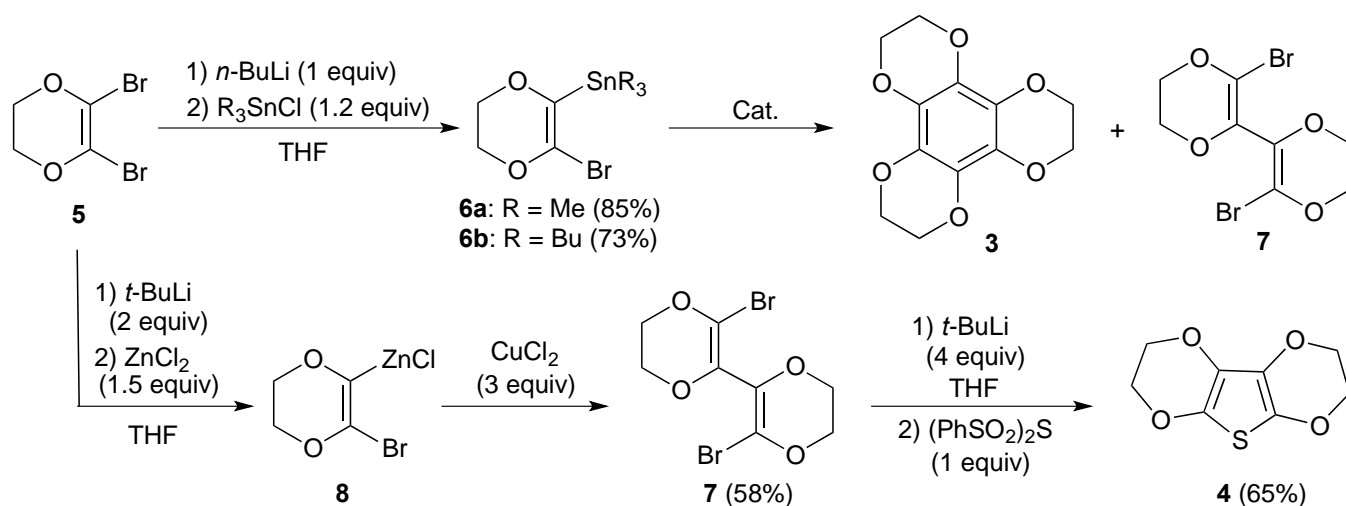
Scheme 1. Synthesis of tris(ethylenedioxy)benzene ( 3 ) and bis(ethylenedioxy)thiophene ( 4 )
