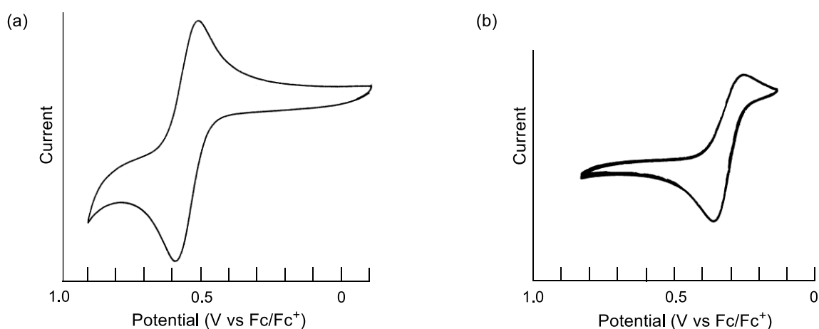
Figure 4. Cyclic voltammograms of 3 (a) and 4 (b): 0.1\text{M} Bu 4 NClO 4 in MeCN under argon at room temperature, Pt working and counter electrodes, scan rate 50\text{ mV s}^{-1} .
