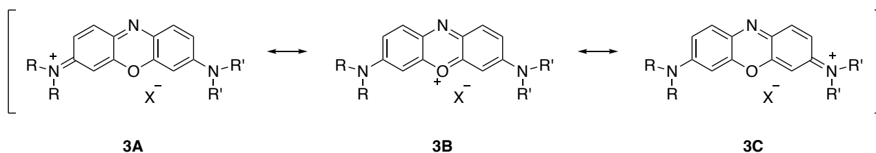
Figure 2. Resonance structures of phenoxazininium salts 3
