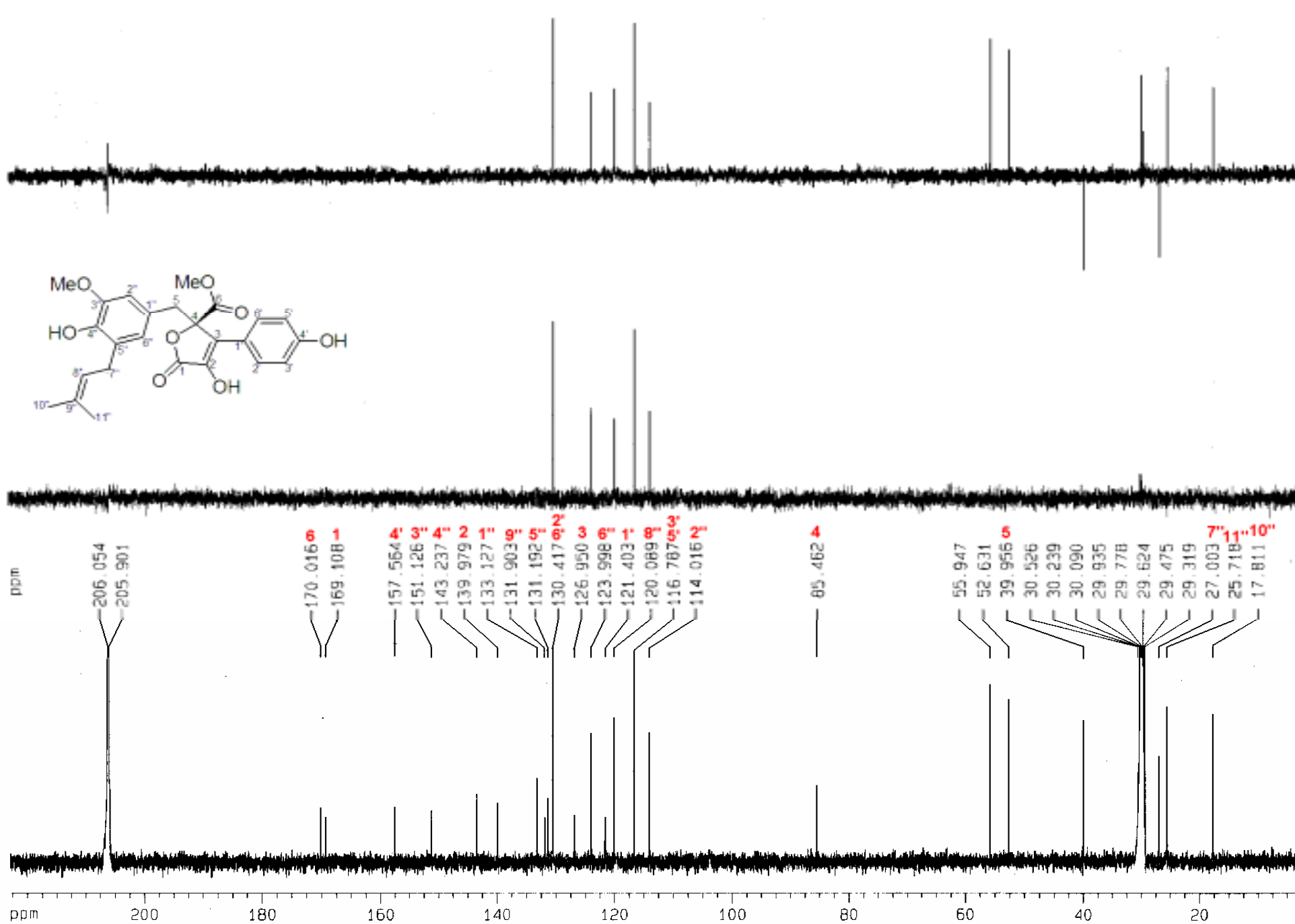
Figure S1. 13 C NMR and DEPT spectra of terrephenol A (1)
