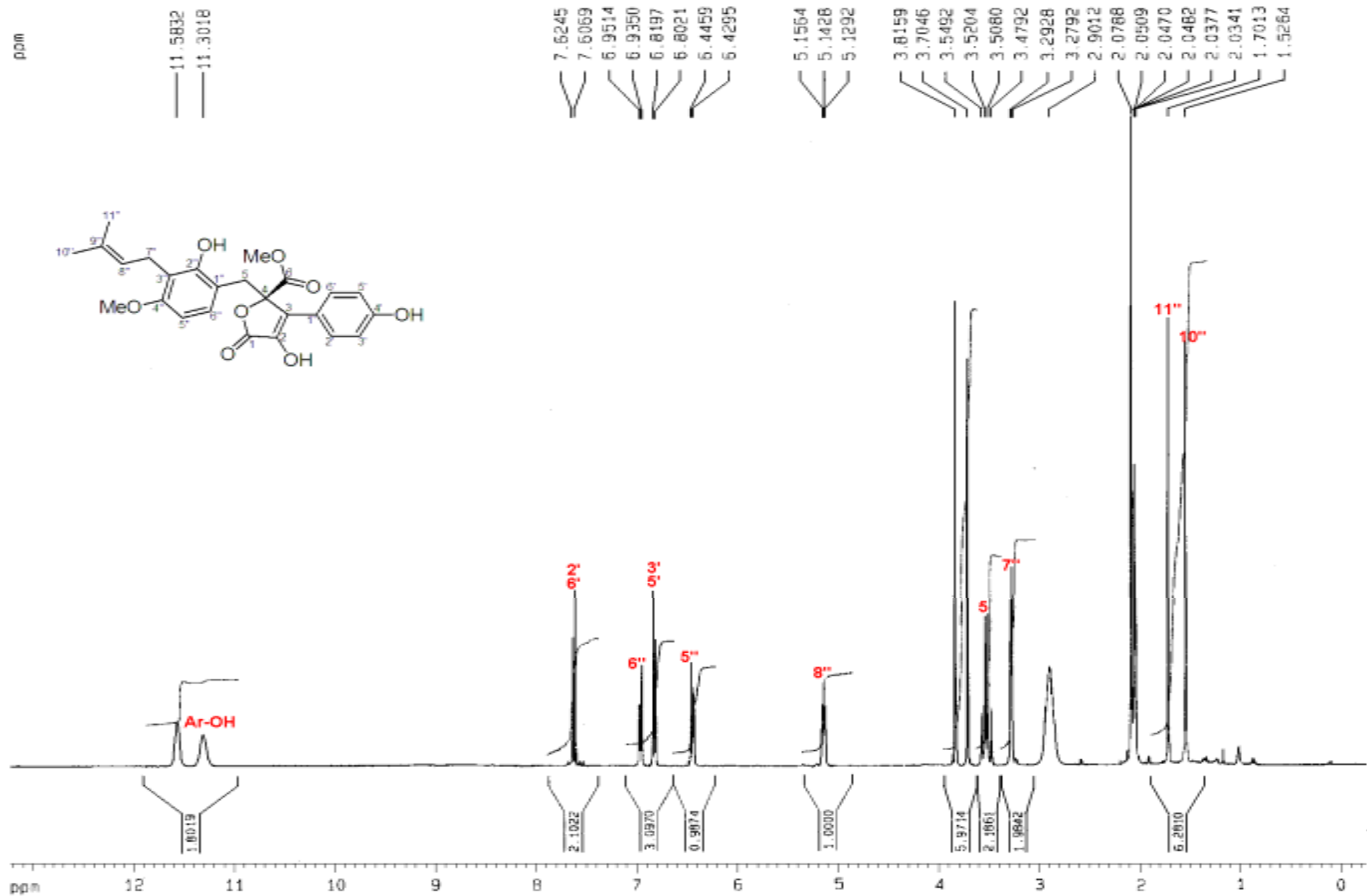
Figure S4. ^1\text{H} NMR spectra of terrephenol B (2)
