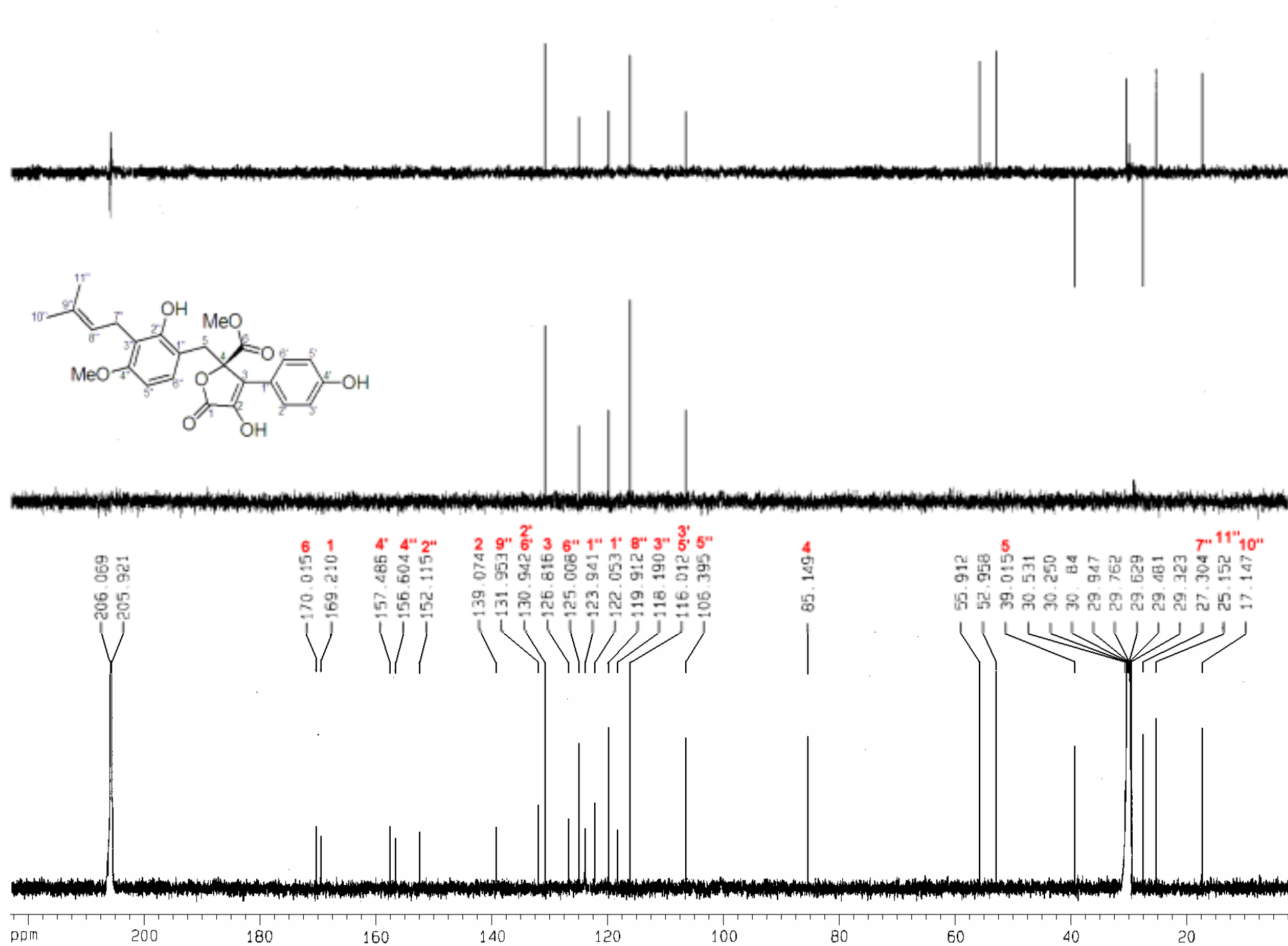
Figure S3. 13 C NMR and DEPT spectra of terrephenol B (2)
