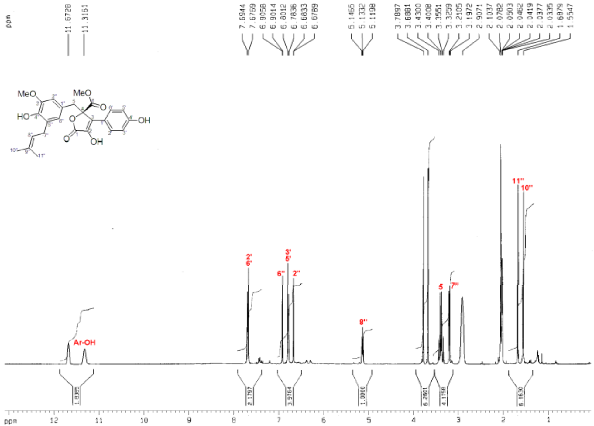
Figure S2. 1 H NMR spectra of terrephenol A (1)
