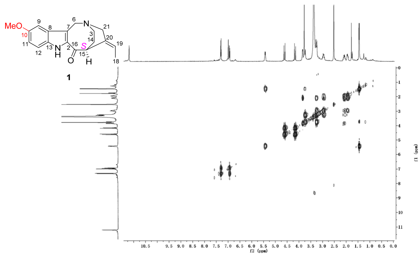
Figure S5. ^1\text{H} - ^1\text{H} COSY spectrum of 10-methoxyconolidine ( 1 ) in \text{DMSO-}d_6 .
