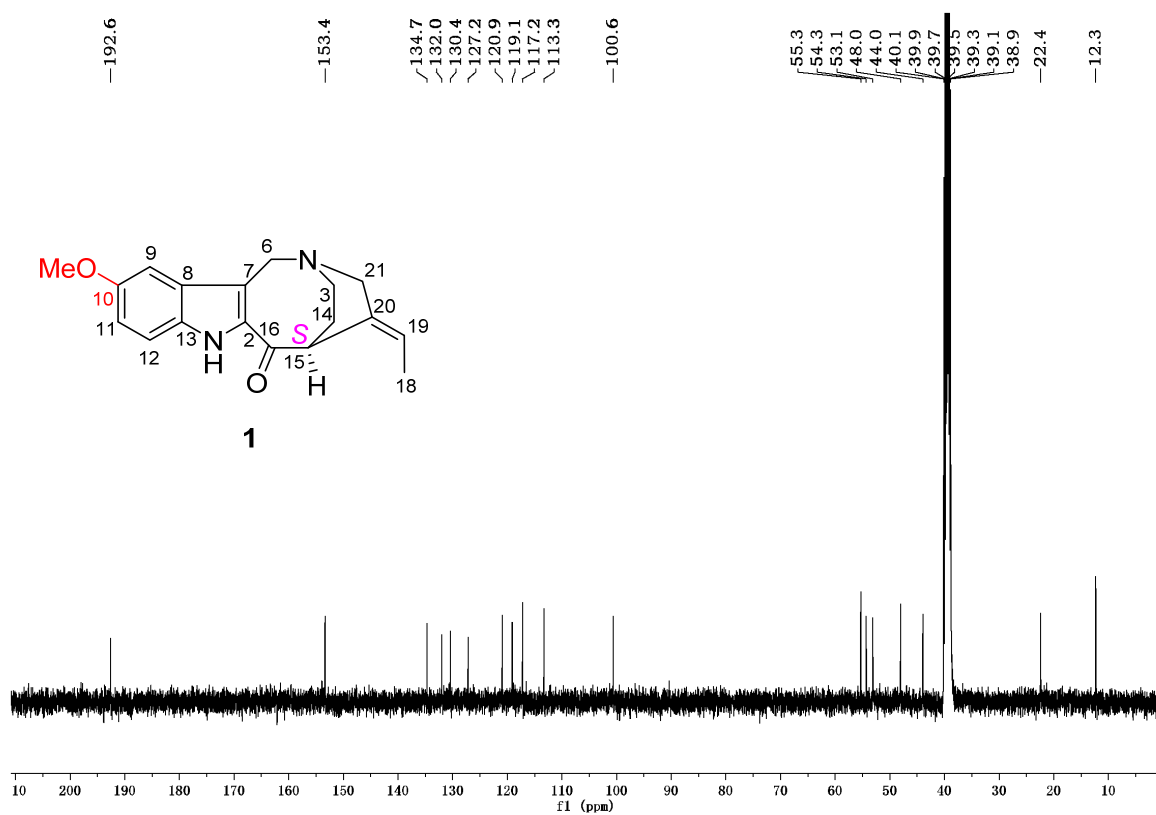
Figure S2. ^{13}\text{C-NMR} spectrum of 10-methoxyconolidine (1) in \text{DMSO-}d_6 .
