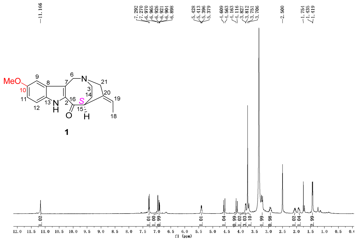
Figure S1. ^1\text{H-NMR} spectrum of 10-methoxyconolidine (1) in \text{DMSO-}d_6 .
