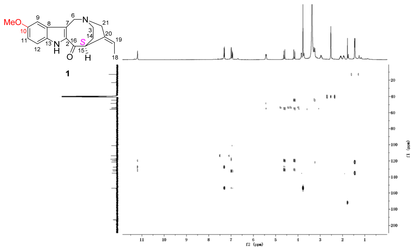
Figure S4. HMBC spectrum of 10-methoxyconolidine ( 1 ) in DMSO- d_6 .
