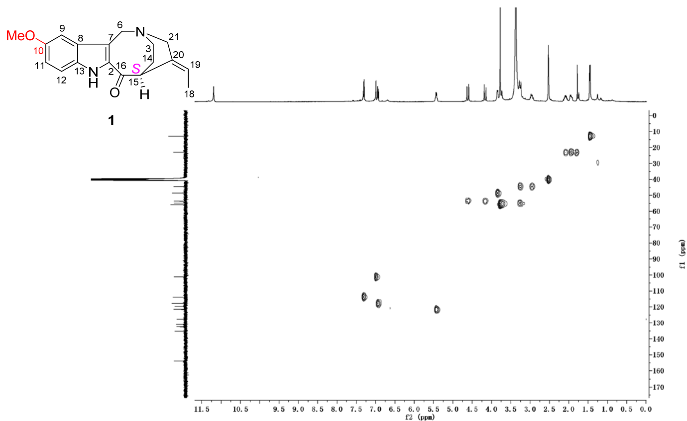
Figure S3. HSQC spectrum of 10-methoxyconolidine ( 1 ) in DMSO- d_6 .
