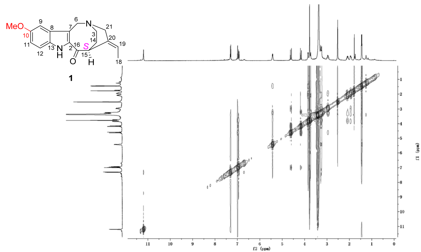
Figure S6. ROESY spectrum of 10-methoxyconolidine ( 1 ) in \text{DMSO-}d_6 .
