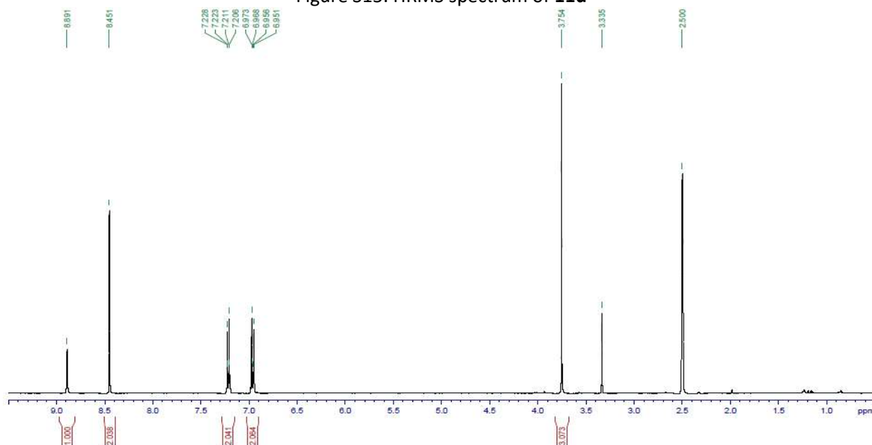
Figure S16. ^1\text{H-NMR} spectrum of 11d measured at 500 MHz in DMSO-d 6
