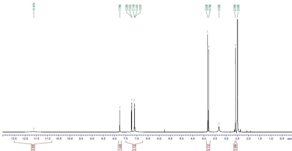
Figure S37. 1 H-NMR spectrum of 16 measured at 500 MHz in DMSO-d 6
