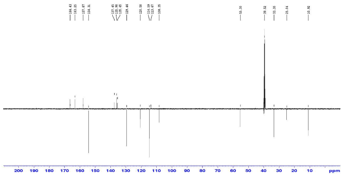
Figure S23. DEPT spectrum of 13b measured at 125 MHz in \text{DMSO-d}_6
