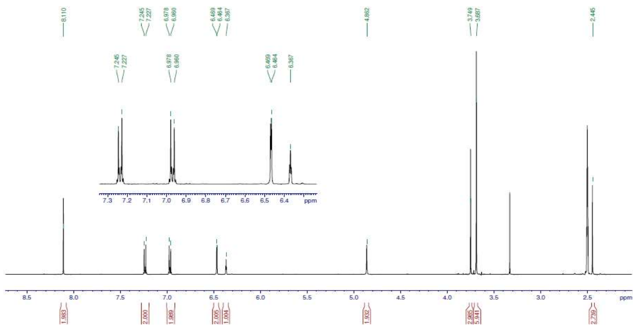
Figure S70. 1 H-NMR spectrum of 25 measured at 500 MHz in DMSO-d 6
