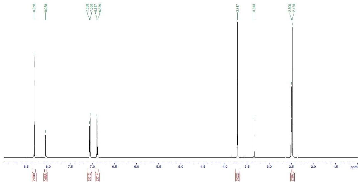
Figure S10. 1 H-NMR spectrum of 11b measured at 500 MHz in DMSO-d 6
