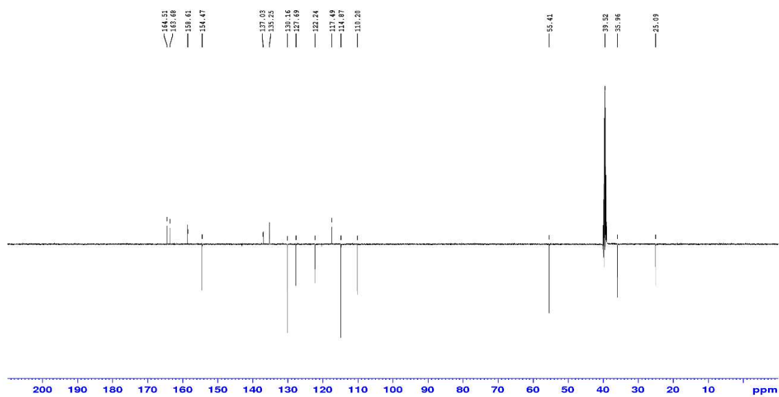
Figure S32. DEPT spectrum of 13e measured at 125 MHz in DMSO- d_6
