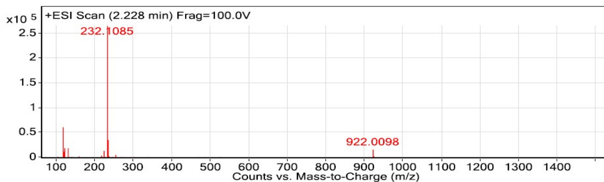
Figure S6. HRMS spectrum of 11a
