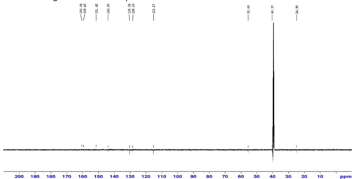
Figure S59. DEPT spectrum of 20 measured at 125 MHz in DMSO-d 6
