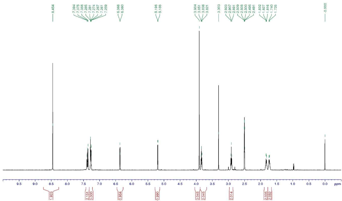
Figure S3. 1 H-NMR spectrum of 7 measured at 400 MHz in DMSO-d 6
