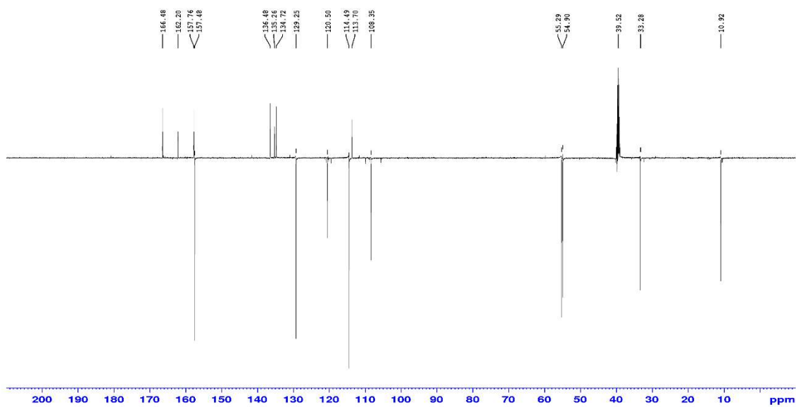
Figure S20. DEPT spectrum of 13a measured at 125 MHz in DMSO- d_6
