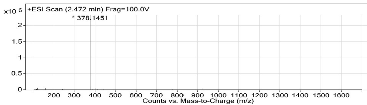
Figure S66. HRMS spectrum of 23
