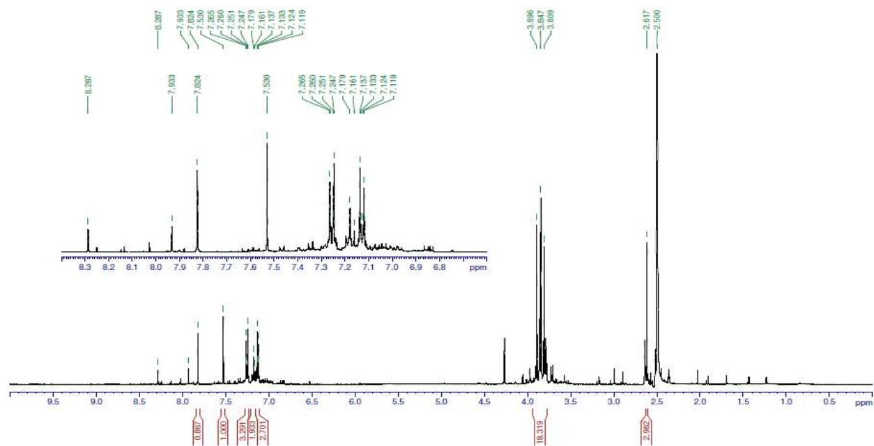
Figure S40. 1 H-NMR spectrum of 17a measured at 500 MHz in DMSO-d 6
