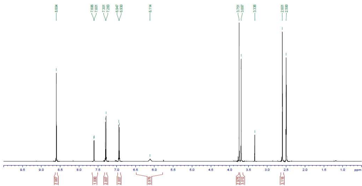
Figure S34. ^1\text{H-NMR} spectrum of 13f measured at 500 MHz in DMSO-d 6
