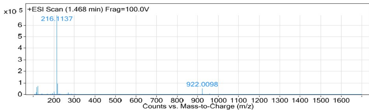
Figure S9. HRMS spectrum of 11b
