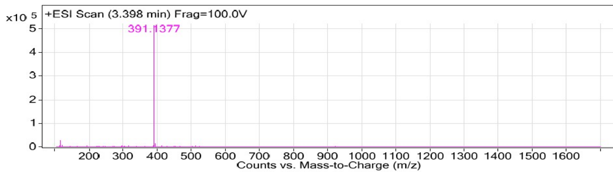
Figure S27. HRMS spectrum of 13d
