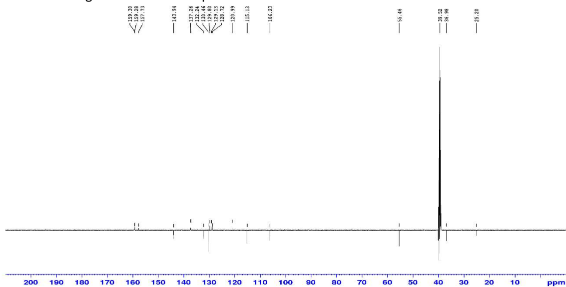
Figure S56. DEPT spectrum of 19 measured at 125 MHz in DMSO-d 6
