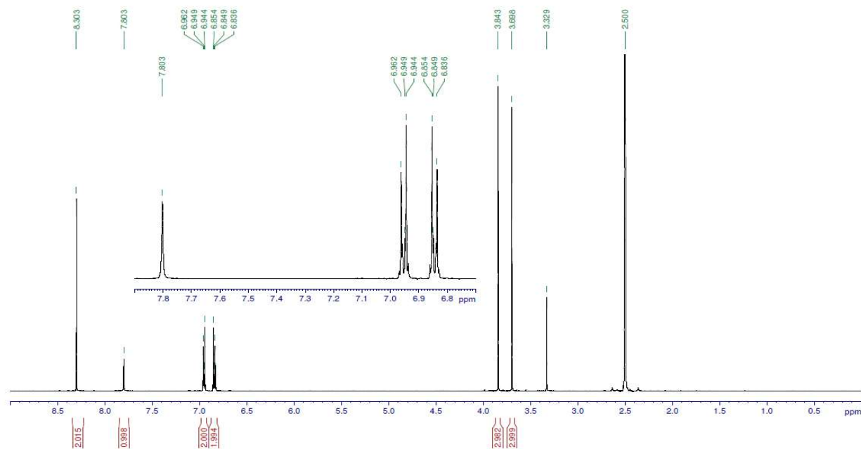
Figure S7. 1 H-NMR spectrum of 11a measured at 500 MHz in DMSO-d 6
