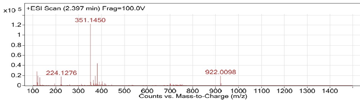
Figure S39. HRMS spectrum of 17a
