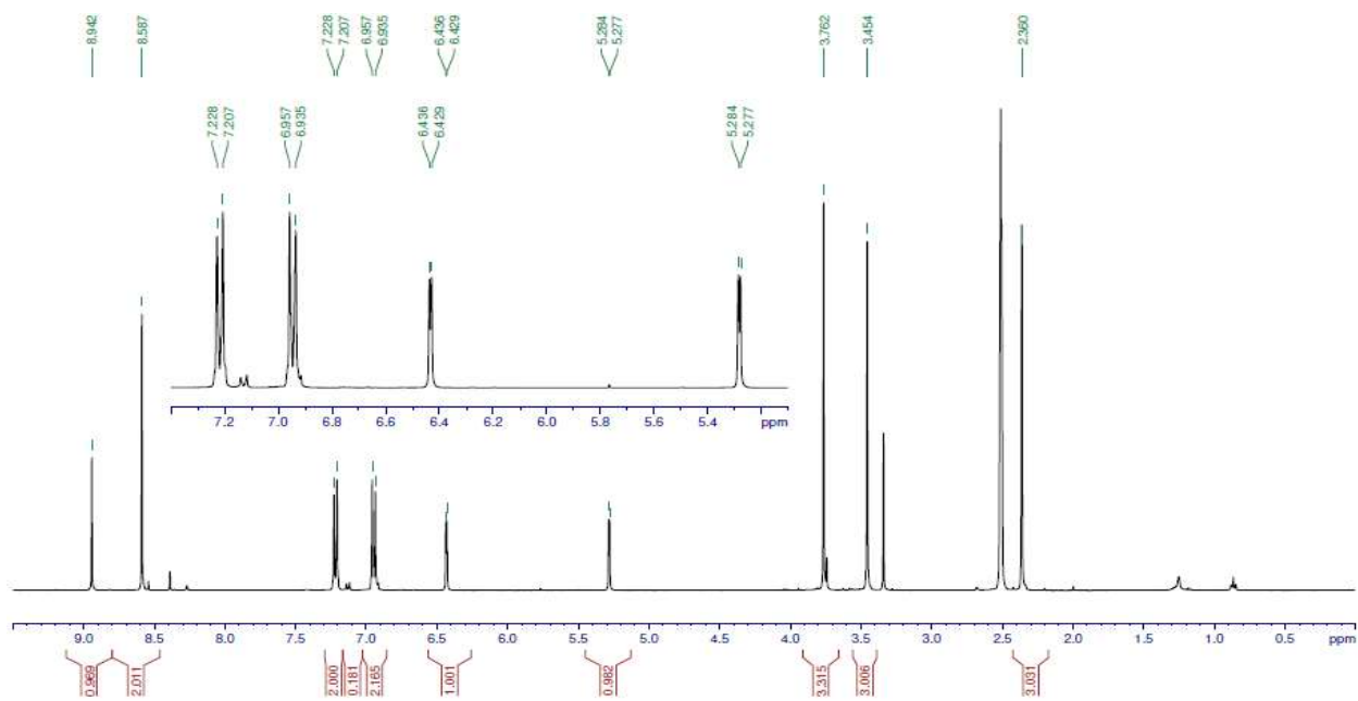
Figure S25. ^1\text{H-NMR} spectrum of 13c measured at 500 MHz in \text{DMSO-d}_6
