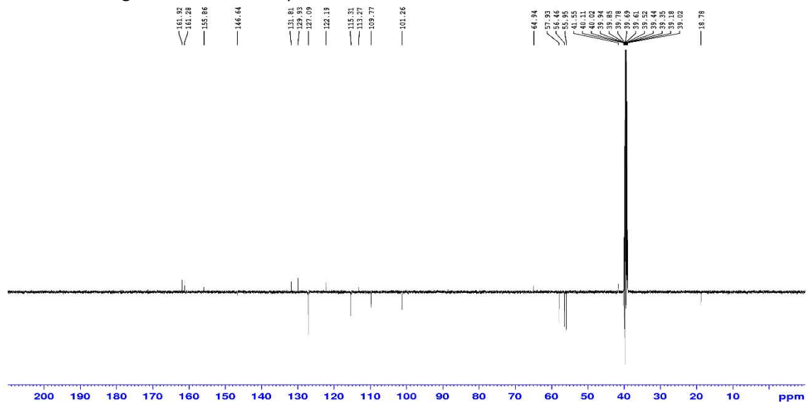
Figure S74. DEPT spectrum of 27 measured at 125 MHz in DMSO-d 6
