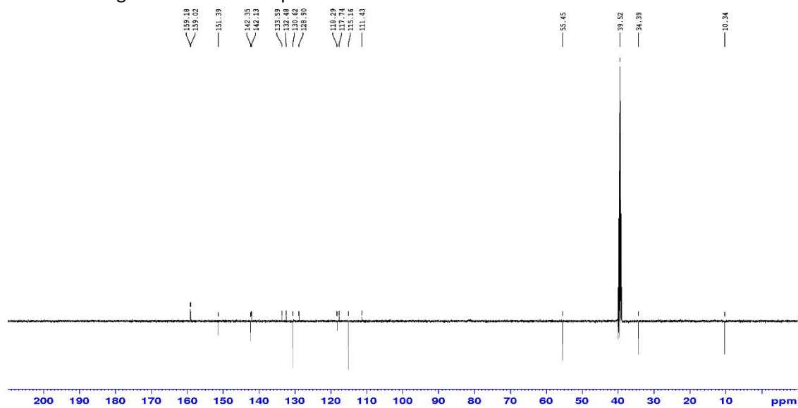
Figure S47. DEPT spectrum of 17c measured at 125 MHz in DMSO-d 6
