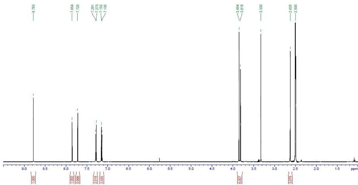
Figure S46. 1 H-NMR spectrum of 17c measured at 500 MHz in DMSO-d 6
