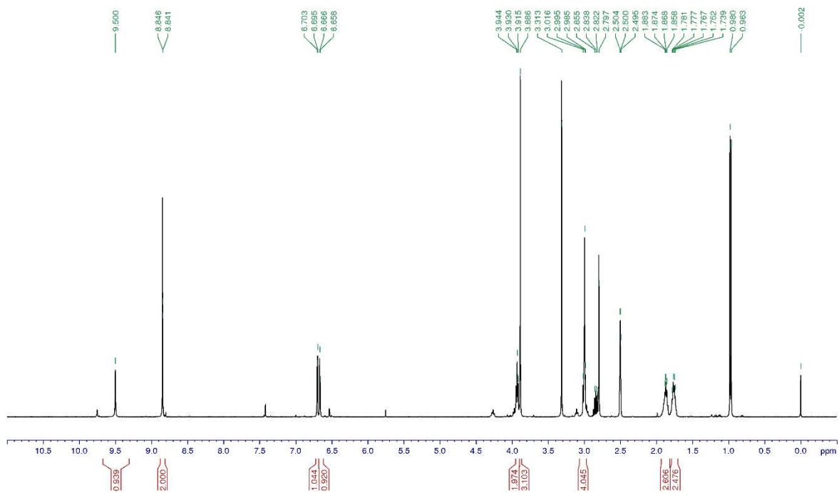
Figure S2. ^1\text{H-NMR} spectrum of 6 measured at 400 MHz in \text{DMSO-d}_6
