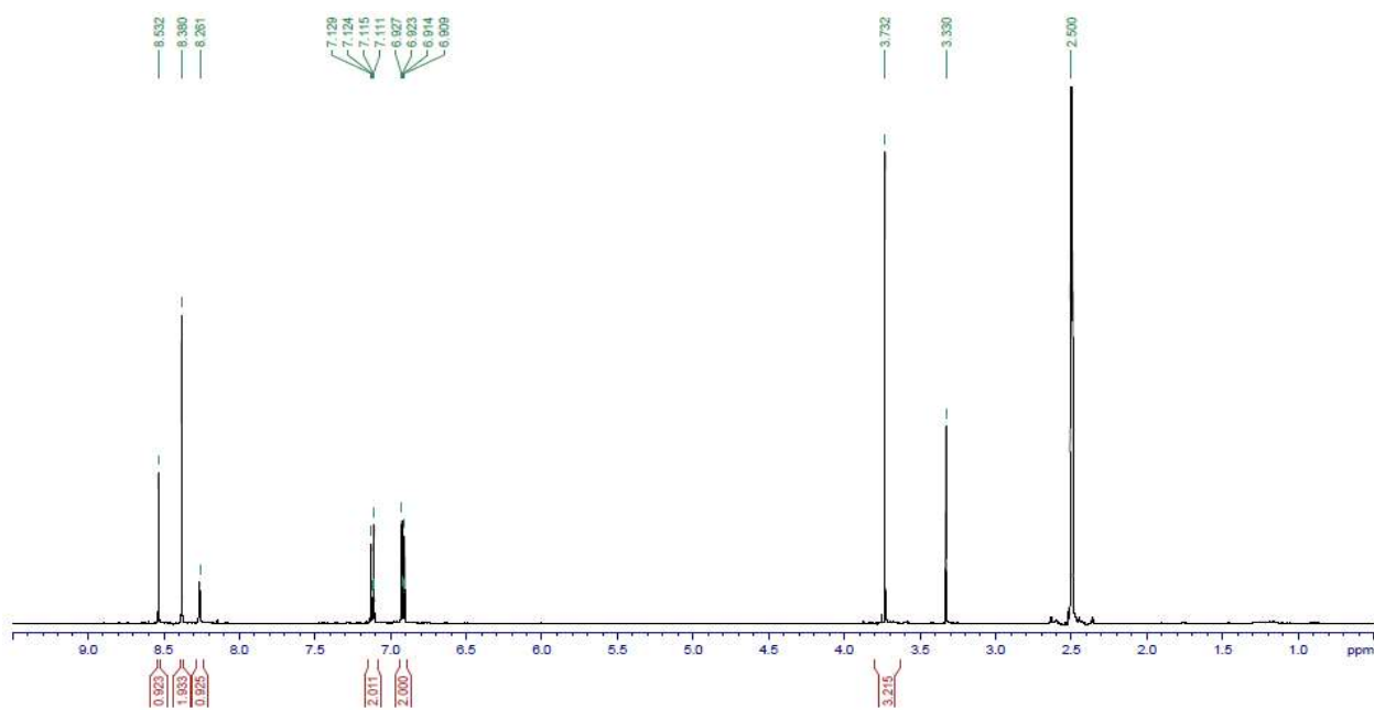
Figure S13. ^1\text{H-NMR} spectrum of 11c measured at 500 MHz in \text{DMSO-d}_6
