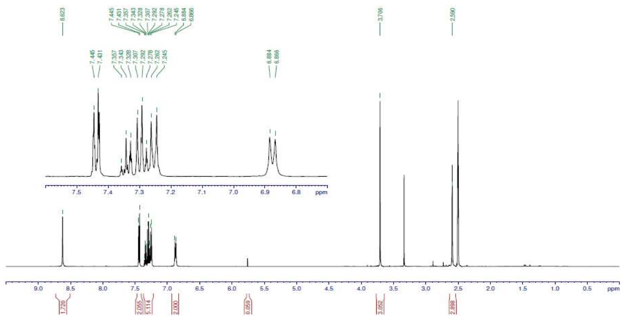
Figure S61. ^1\text{H-NMR} spectrum of 22a measured at 500 MHz in DMSO-d 6
