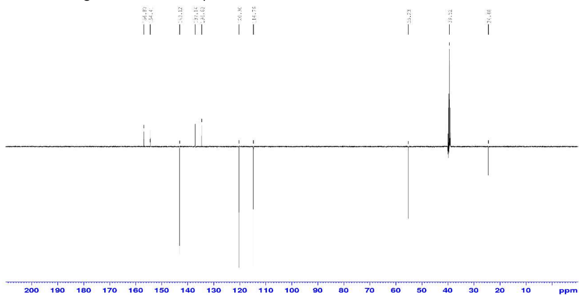
Figure S11. DEPT spectrum of 11b measured at 125 MHz in DMSO-d 6
