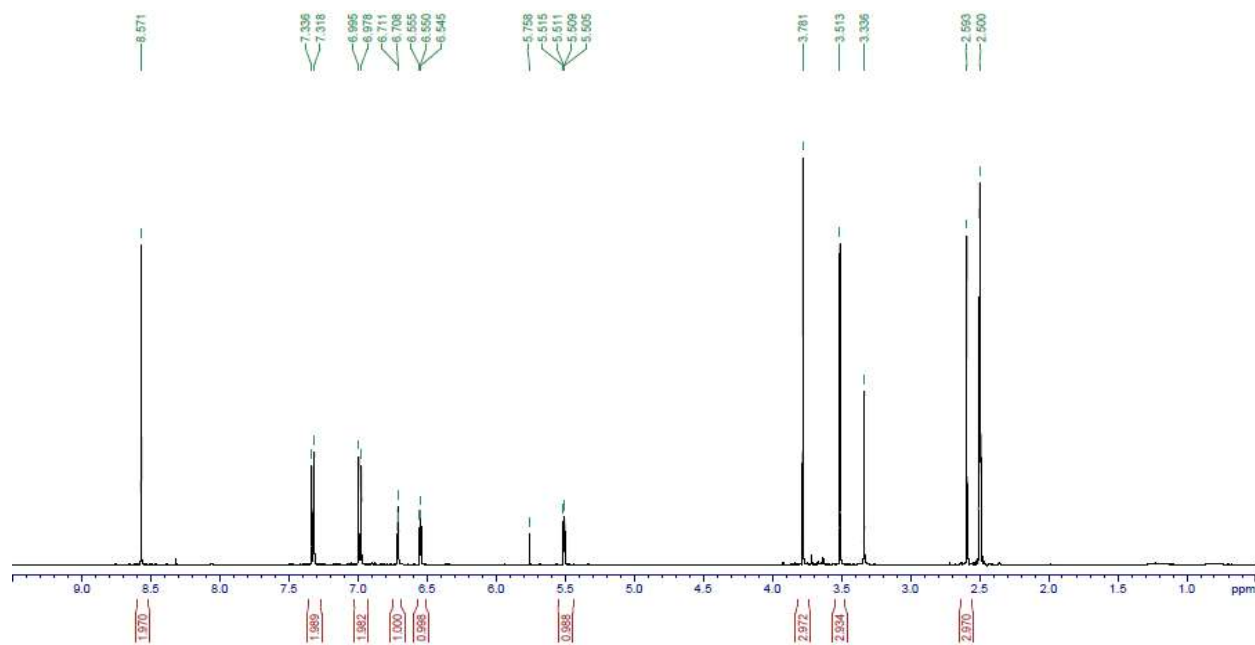
Figure S31. ^1\text{H} -NMR spectrum of 13e measured at 500 MHz in DMSO- d_6
