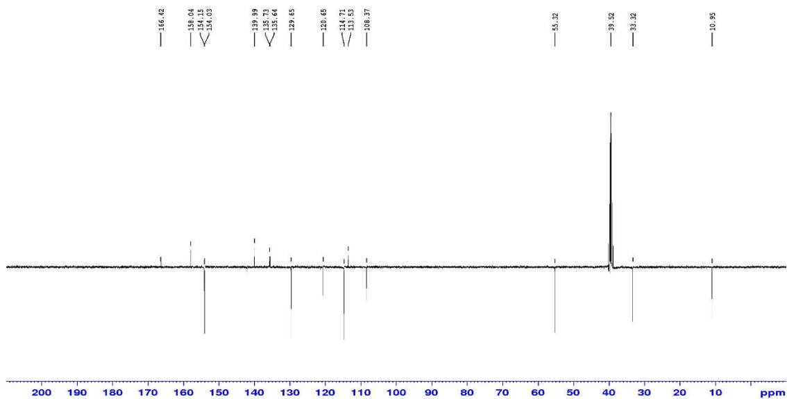
Figure S26. DEPT spectrum of 13c measured at 100 MHz in \text{DMSO-d}_6
