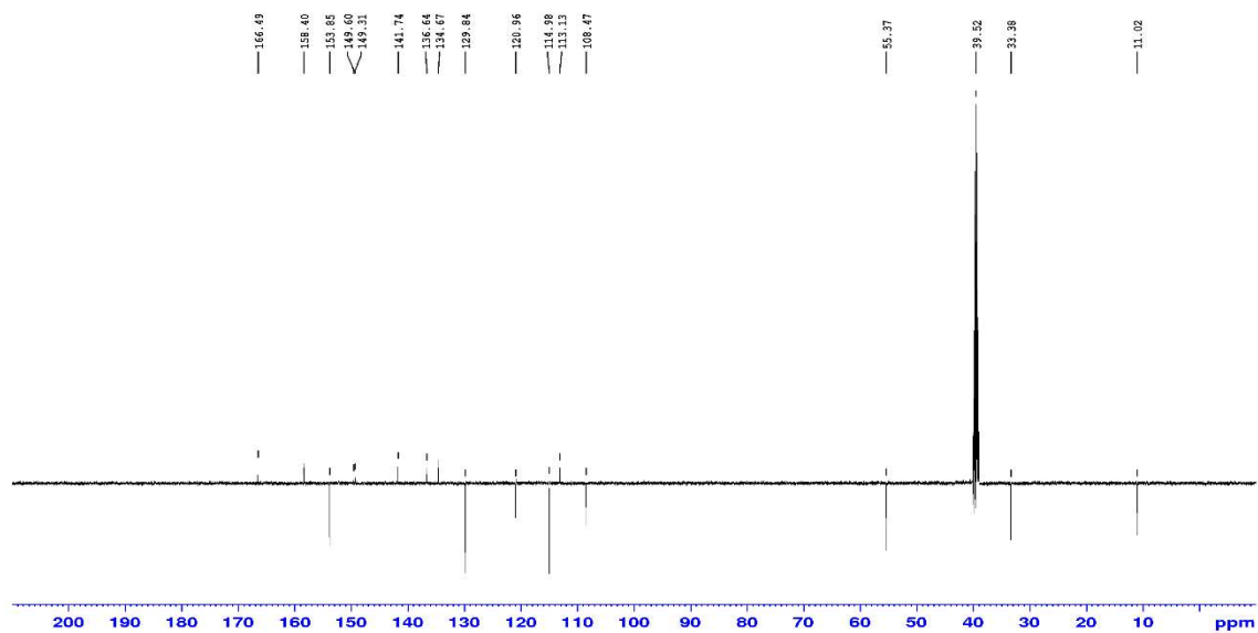
Figure S29. DEPT spectrum of 13d measured at 125 MHz in DMSO-d 6
