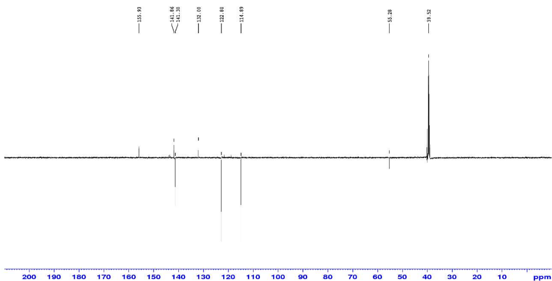
Figure S17. DEPT spectrum of 11d measured at 100 MHz in DMSO-d 6
