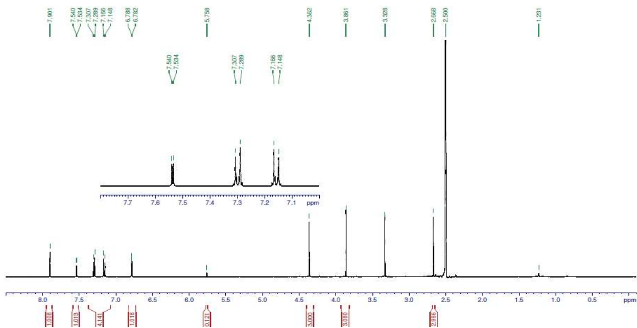
Figure S55. 1 H-NMR spectrum of 19 measured at 500 MHz in DMSO-d 6
