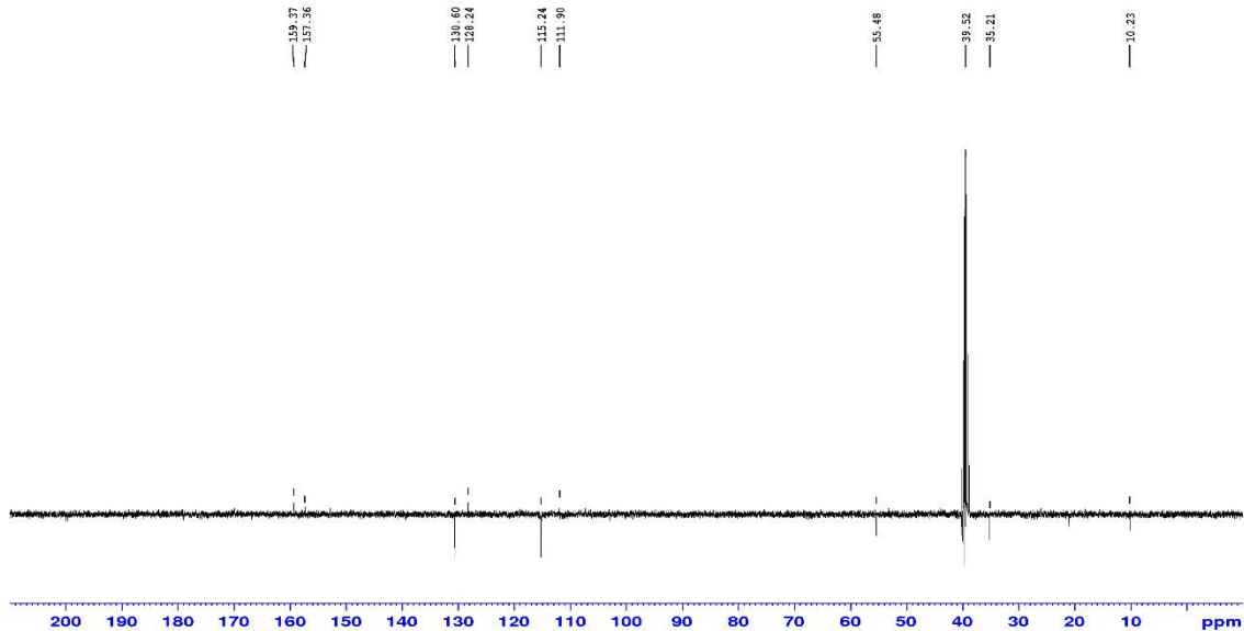
Figure S38. DEPT spectrum of 16 measured at 125 MHz in DMSO-d 6
