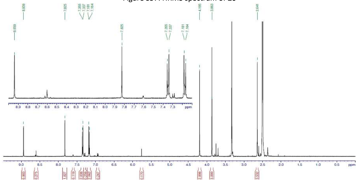
Figure S58. 1 H-NMR spectrum of 20 measured at 500 MHz in DMSO-d 6
