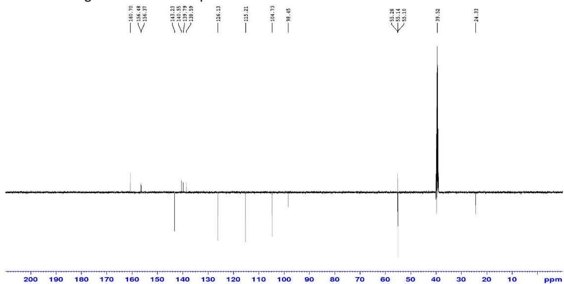
Figure S71. DEPT spectrum of 25 measured at 125 MHz in DMSO-d 6
