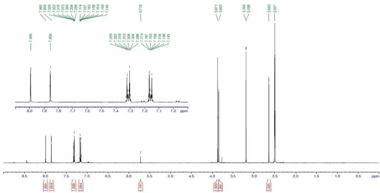
Figure S49. 1 H-NMR spectrum of 17d measured at 500 MHz in DMSO-d 6
