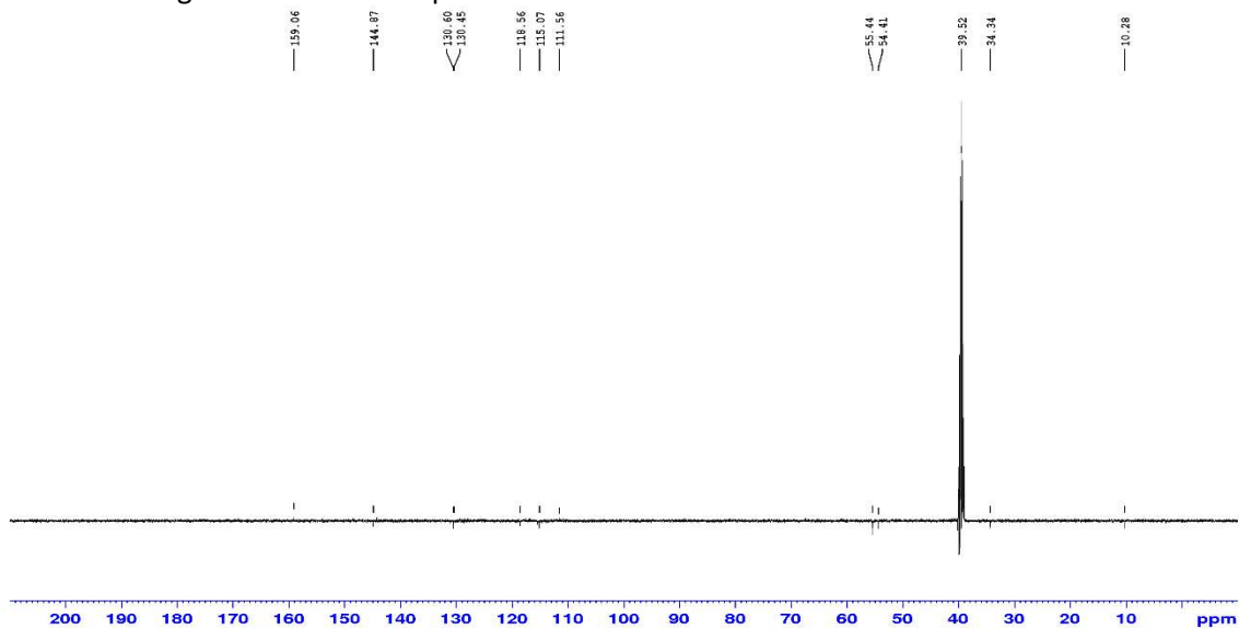
Figure S41. DEPT spectrum of 17a measured at 125 MHz in DMSO-d 6
