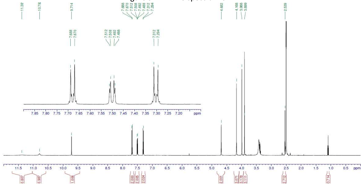
Figure S73. 1 H-NMR spectrum of 27 measured at 500 MHz in DMSO-d 6
