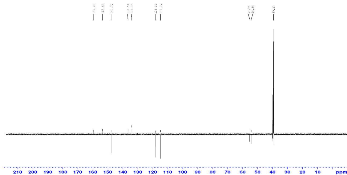
Figure S8. DEPT spectrum of 11a measured at 125 MHz in DMSO-d 6
