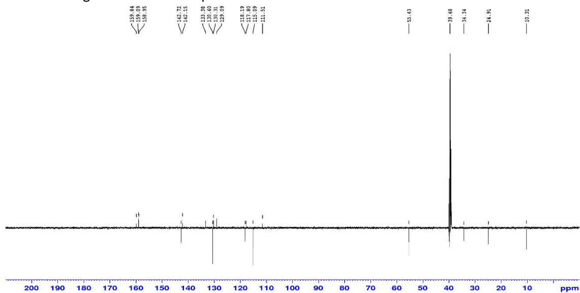
Figure S44. DEPT spectrum of 17b measured at 125 MHz in DMSO-d 6
