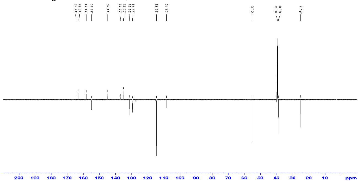
Figure S35. DEPT spectrum of 13f measured at 125 MHz in DMSO-d 6
