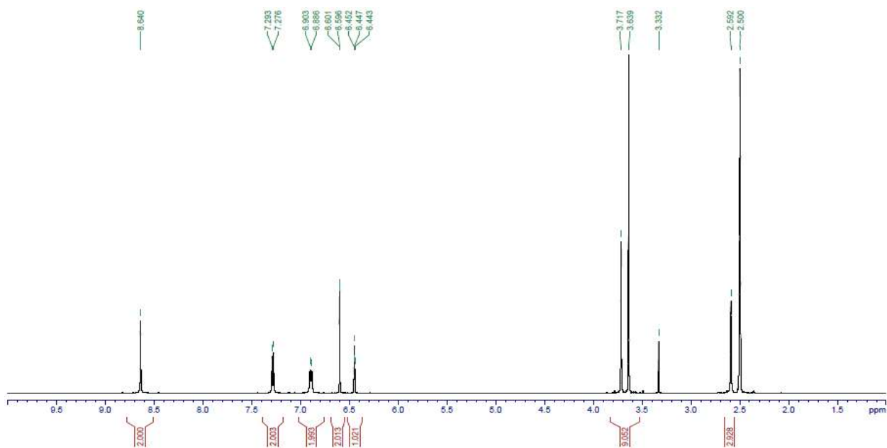
Figure S64. 1 H-NMR spectrum of 22b measured at 500 MHz in DMSO-d 6
