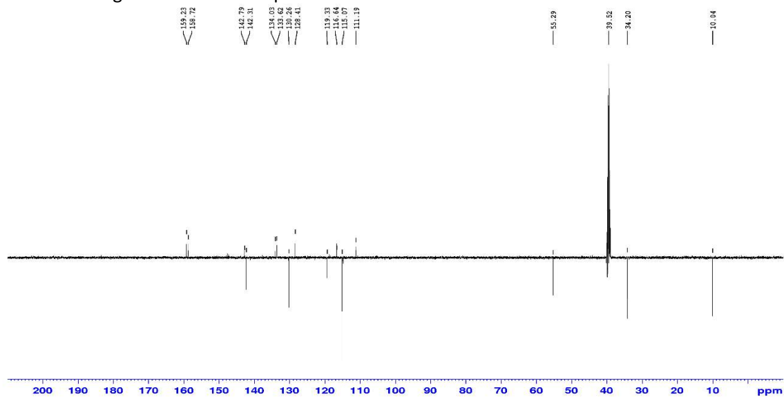
Figure S50. DEPT spectrum of 17d measured at 125 MHz in DMSO-d 6
