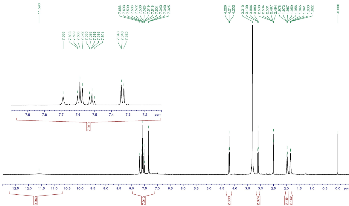
Figure S5. ^1\text{H-NMR} spectrum of 8 measured at 400 MHz in \text{DMSO-d}_6
