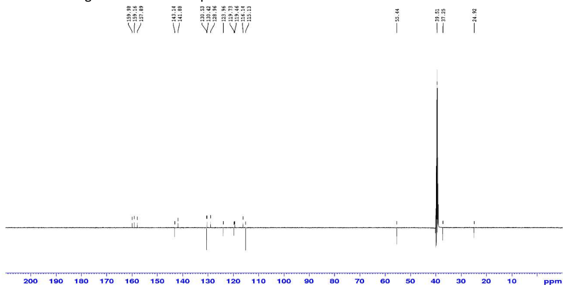
Figure S53. DEPT spectrum of 18 measured at 125 MHz in DMSO-d 6
