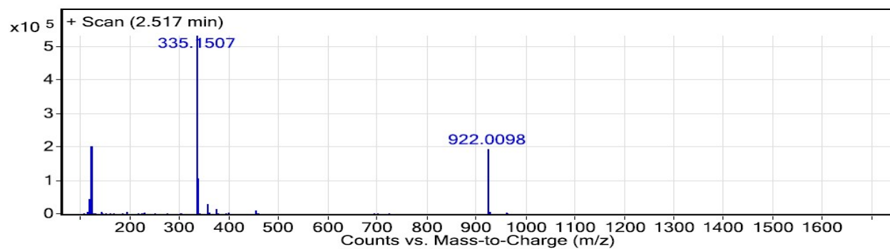
Figure S42. HRMS spectrum of 17b
