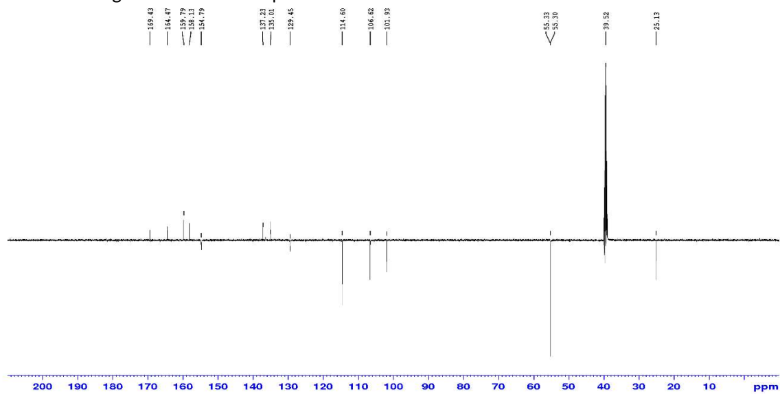
Figure S65. DEPT spectrum of 22b measured at 125 MHz in DMSO-d 6
