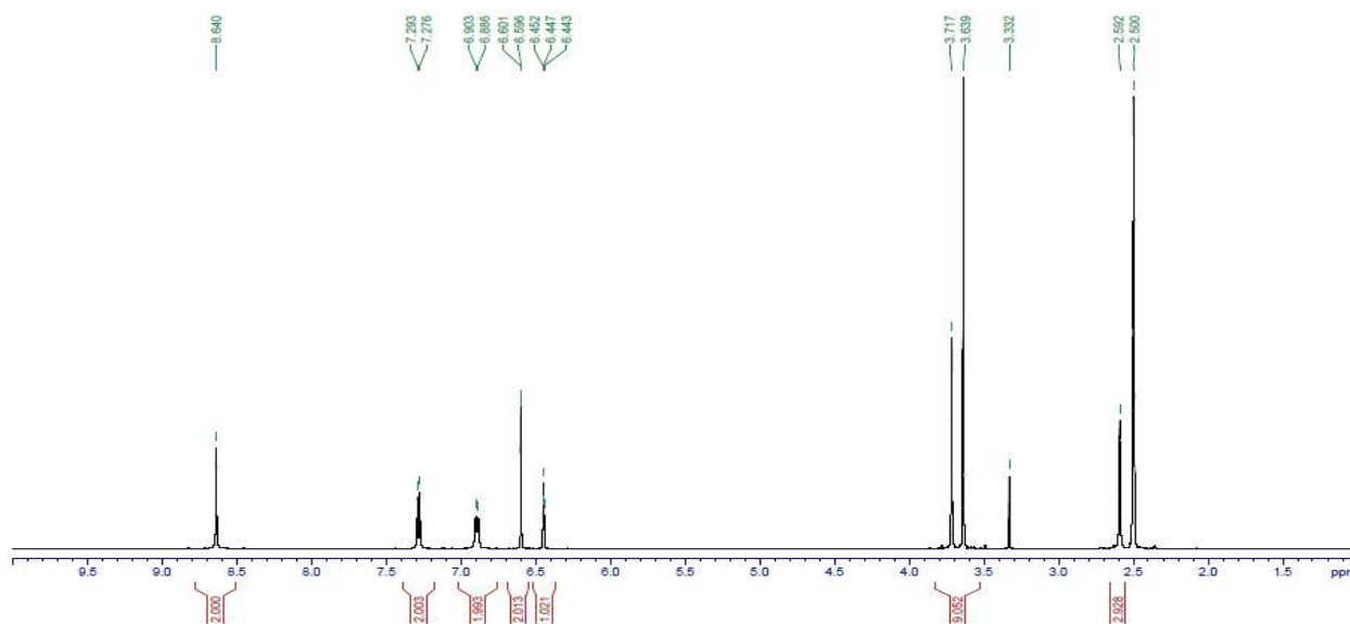
Figure S67. 1 H-NMR spectrum of 23 measured at 500 MHz in DMSO-d 6
