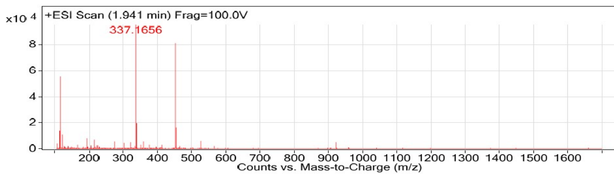
Figure S21. HRMS spectrum of 13b
