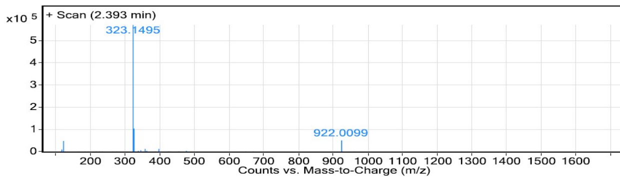
Figure S30. HRMS spectrum of 13e
