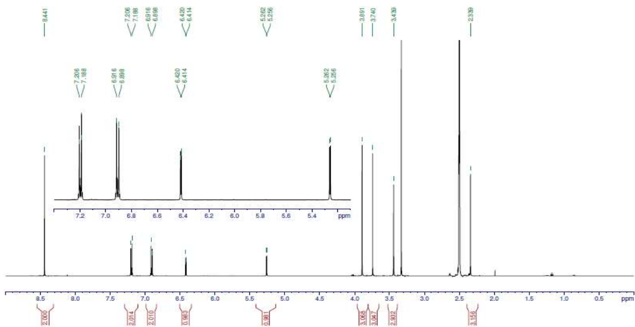
Figure S19. ^1\text{H-NMR} spectrum of 13a measured at 500 MHz in DMSO- d_6
