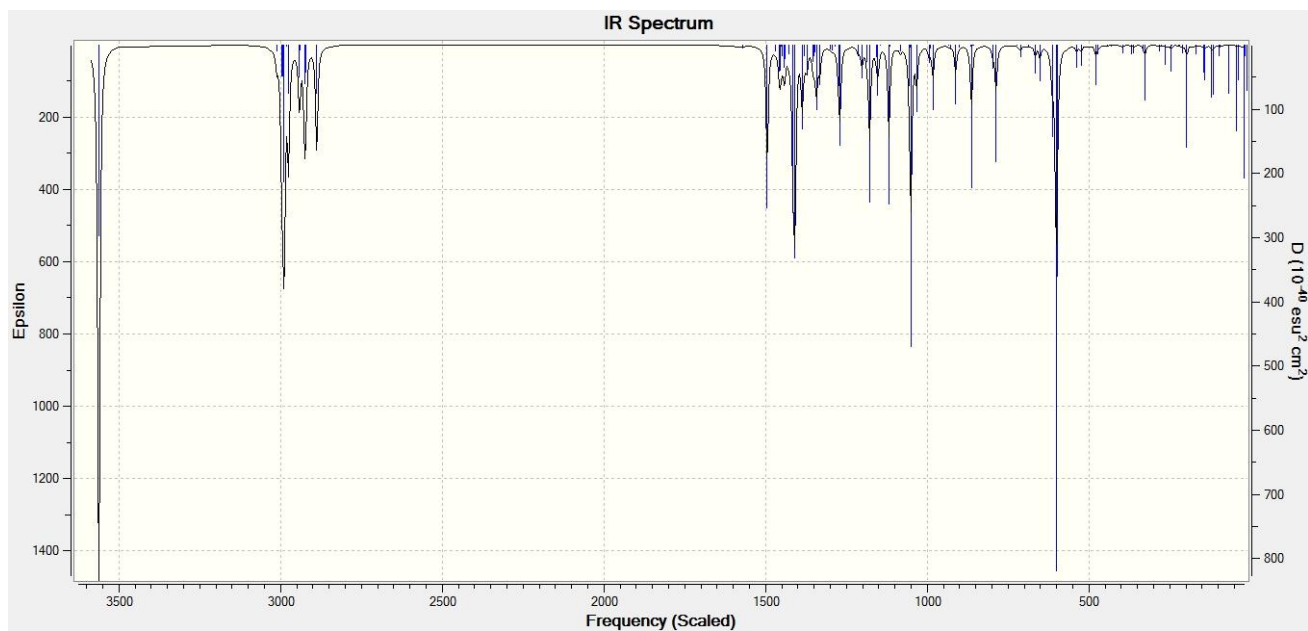
Figure S1. Theoretical FTIR spectrum of bipyrazolic compound 2
