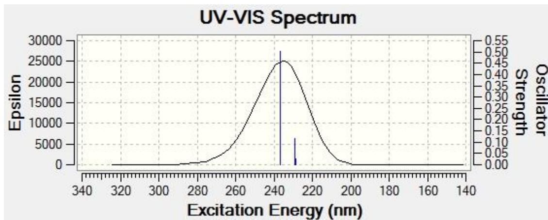
Figure S2. Theoretical UV-Visible spectrum of bipyrazolic compound 2
