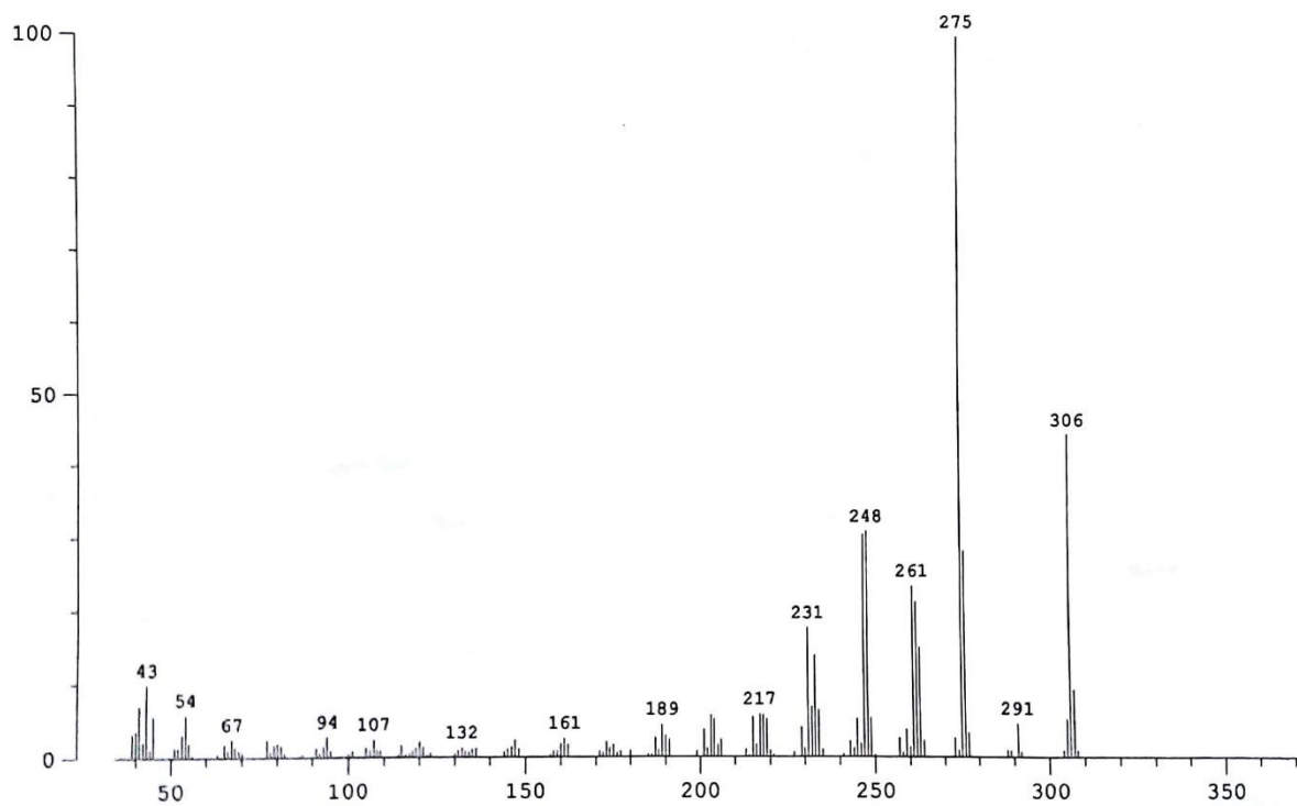
Figure S5. Mass spectrum of bipyrzolic compound 2
