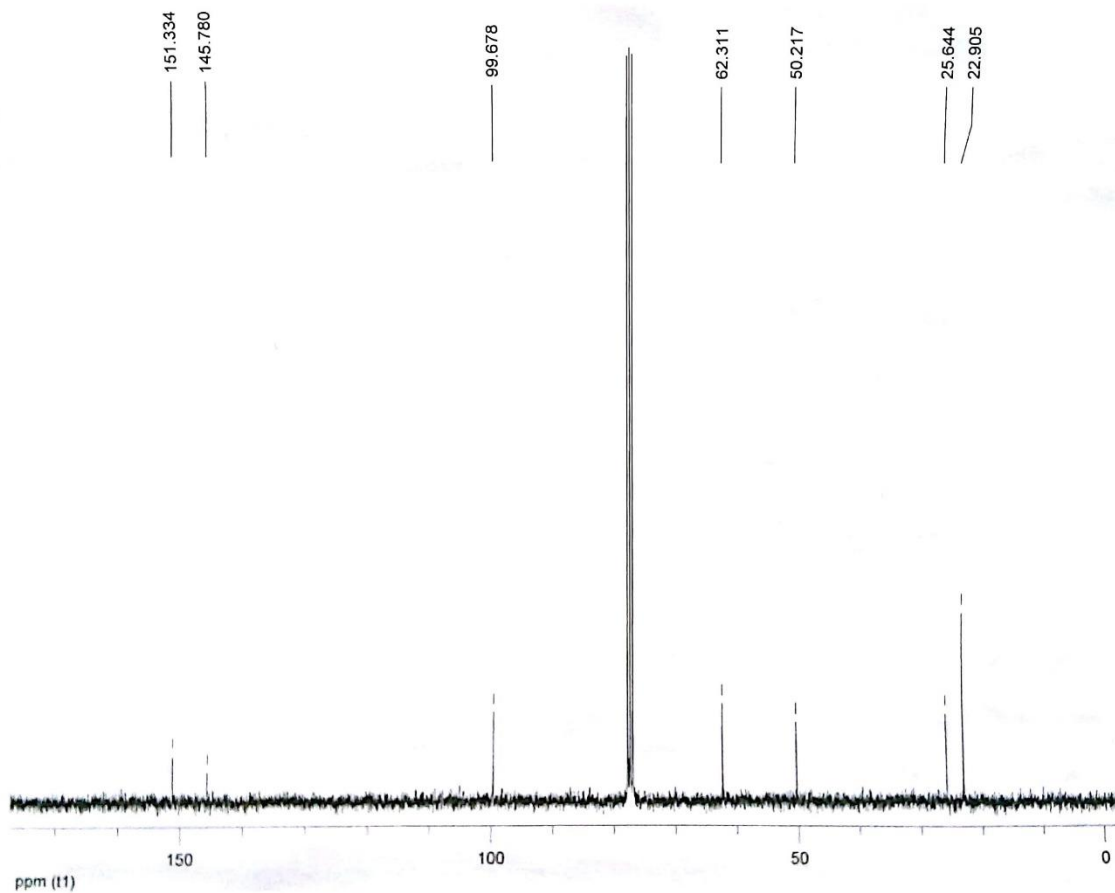
Figure S4. 13 C NMR spectrum of compound 2
