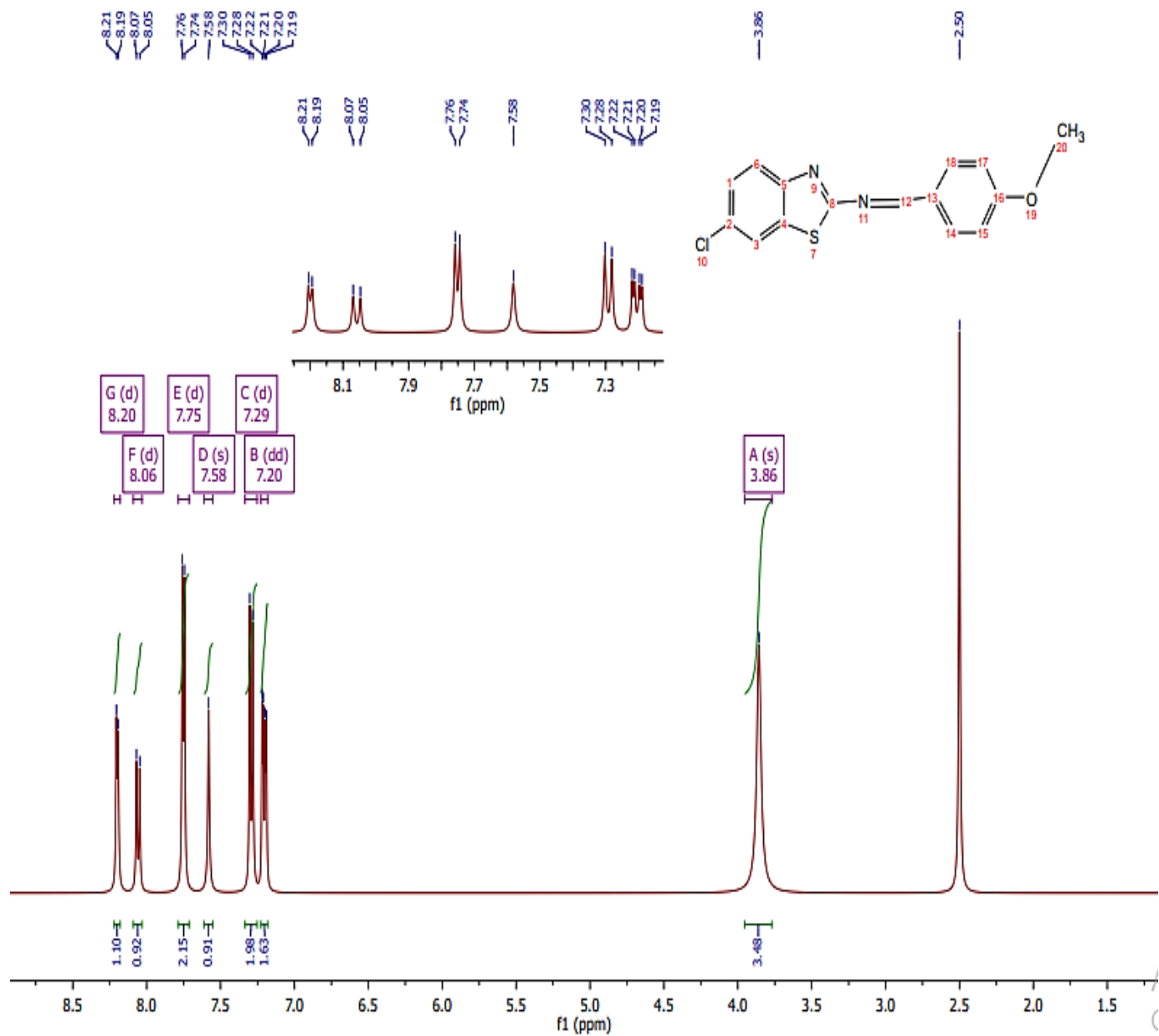
Fig 1: The 1 H NMR spectrum of compound 3b in DMSO-d 6 solvent
