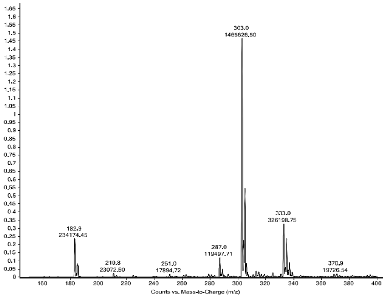
Fig 2: The Mass spectrum of compound 3b
