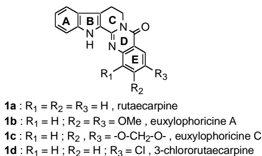
Figure 1. Rutaecarpine alkaloids
