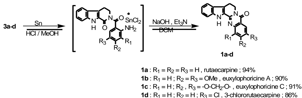
Scheme 4. One-pot reductive-cyclization synthesis of 1a-d
