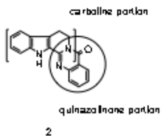
Figure 2. Quinazolinocarboline backbone
