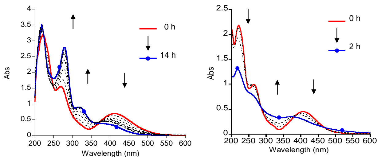
Figure 3. Absorption spectra change of 1b by irradiation of 254 nm light in MeOH (left) and in n -hexane (right), 1.5 \times 10^{-4} M
