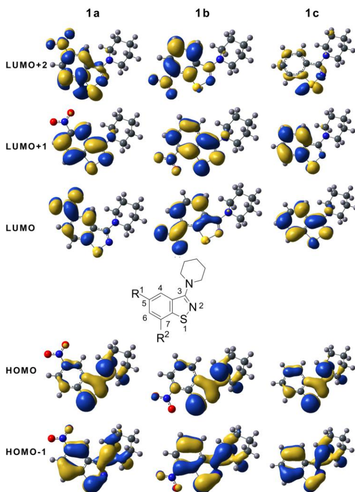
Figure 9. Molecular orbitals of 1a , 1b , and 1c obtained by TD-DFT B3LYP/6-31++G(d) method
