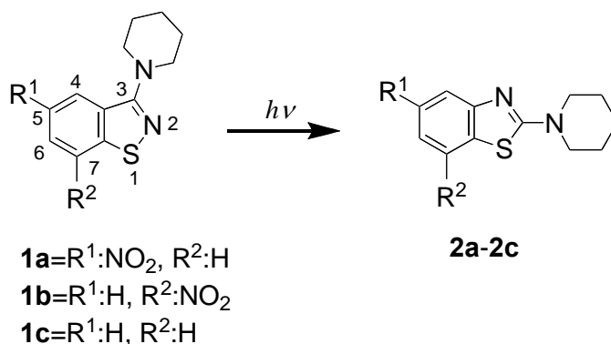
Figure 1. Photochemical isomerization of 3-piperidino-1,2-benzisothiazole derivatives ( 1a-c ) to benzothiazole derivatives ( 2a-c )
