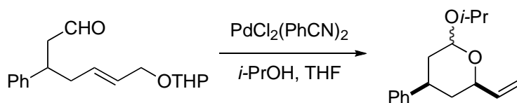
Scheme 1. Palladium(II)-catalyzed cyclization of the aldehyde
