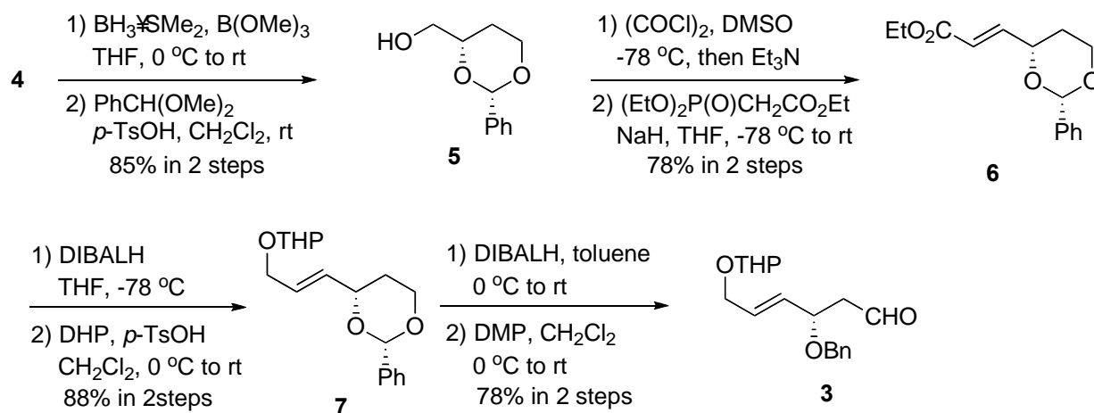
Scheme 3. Preparation of the aldehyde 3
