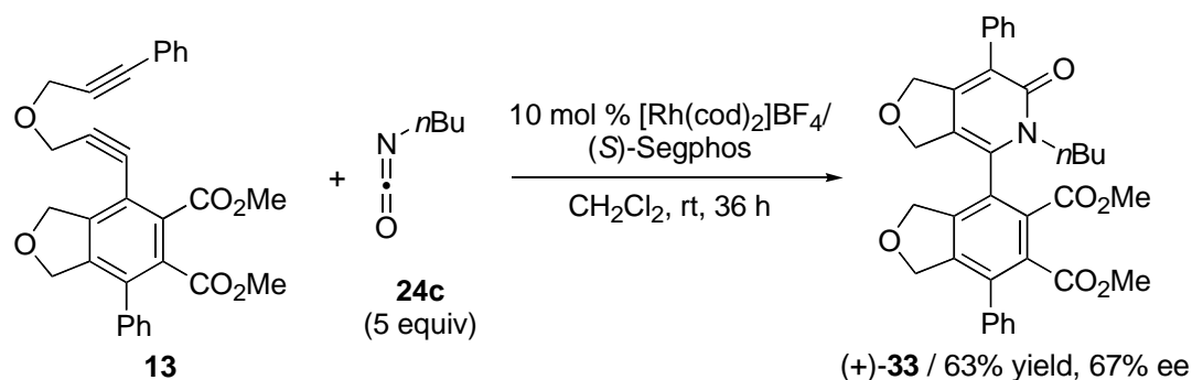
Scheme 30. Cationic Rhodium(I)/Segphos Complex-Catalyzed Atropselective [2+2+2] Cycloaddition of 1,6-Diynes with Isocyanate
