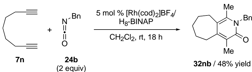
Scheme 29. Cationic Rhodium(I)/H 8 -BINAP Complex-Catalyzed [2+2+2] Cycloaddition of 1,8-Diyne with Isocyanate
