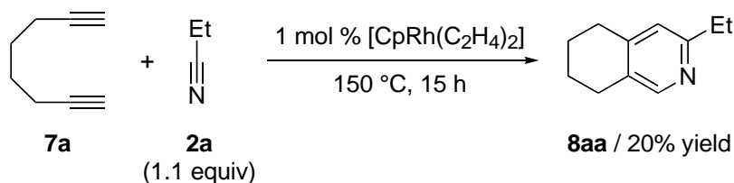
Scheme 6. Rhodium(I)/Cp Complex-Catalyzed [2+2+2] Cycloaddition of 1,7-Diyne with Nitrile
