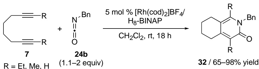
Scheme 28. Cationic Rhodium(I)/H 8 -BINAP Complex-Catalyzed [2+2+2] Cycloaddition of 1,7-Diynes with Isocyanate
