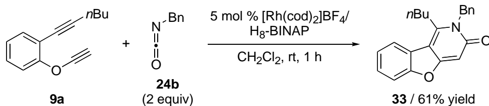
Scheme 27. Cationic Rhodium(I)/H 8 -BINAP Complex-Catalyzed [2+2+2] Cycloaddition of Phenol-Linked 1,6-Diyne with Isocyanate
