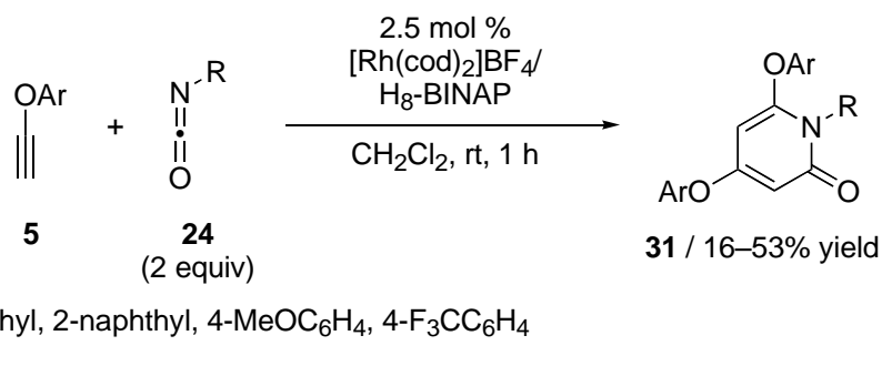
Scheme 26. Cationic Rhodium(I)/H 8 -BINAP Complex-Catalyzed [2+2+2] Cycloaddition of Aryl Ethynyl Ethers with Isocyanates
