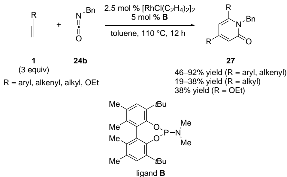
Scheme 23. Neutral Rhodium(I)/Phosphoramidite Complex-Catalyzed [2+2+2] Cycloaddition of Terminal Alkynes with Isocyanates: Alkyne Scope
