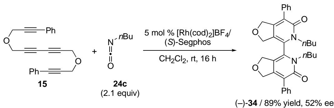
Scheme 31. Cationic Rhodium(I)/Segphos Complex-Catalyzed Atropselective Double [2+2+2] Cycloaddition of Tetrayne with Isocyanate
