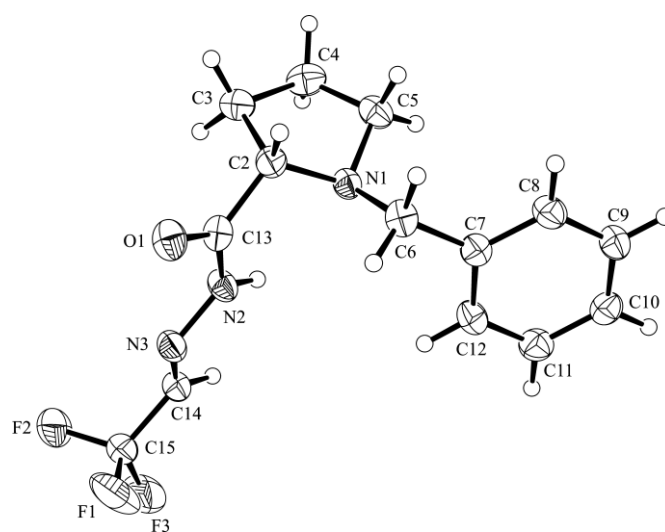
Figure 1. ORTEP plot 7 of the molecular structure of one conformation of 3c (arbitrary numbering of the atoms; 50% probability ellipsoids)
