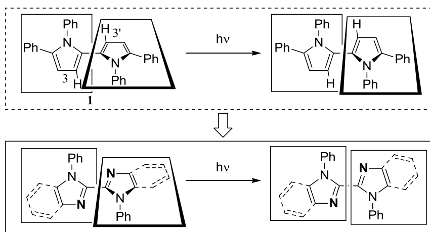
Scheme 1. Proposed representation of the \pi -expansion of the 2,2'-bipyrrole and 2,2'-biimidazole derivatives by photoexcitation
