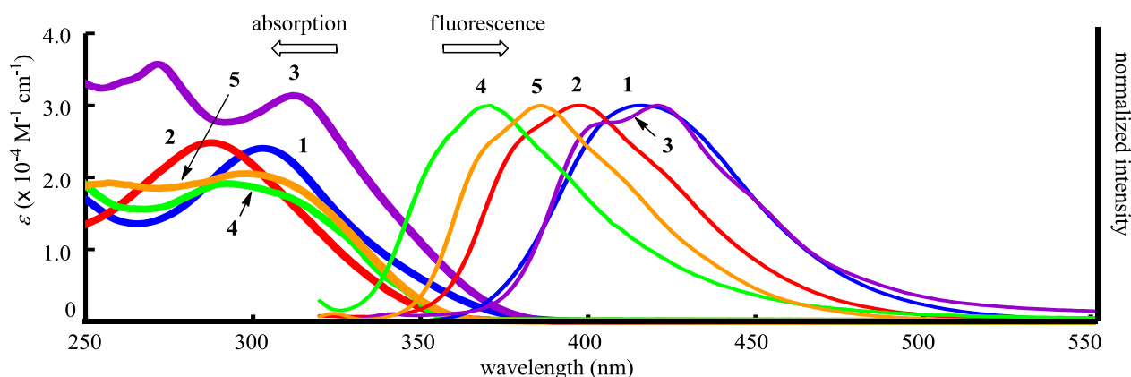
Figure 1. UV-VIS absorption (bold line; 3.0 \times 10^{-5} M in THF) and fluorescence (narrow line; 3.0 \times 10^{-7} M in THF, excited at \lambda_{\max} ) spectra of 1 (blue line), 2 (red line), 3 (purple line), 4 (green line), and 5 (orange line)
