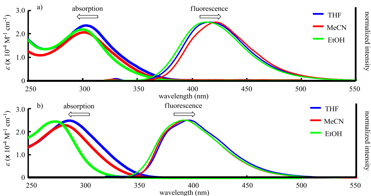
Figure 2. UV-Vis absorption (bold line; 3.0 \times 10^{-5} \text{ M} ) and fluorescence (narrow line; 3.0 \times 10^{-7} \text{ M} , excited at \lambda_{\text{max}} ) spectra of a) 1 and b) 2 in THF (blue line), MeCN (red line), and EtOH (green line)
