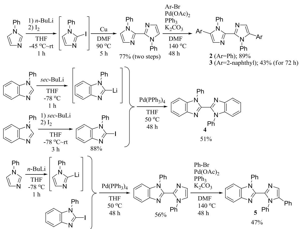
Scheme 2. Synthesis of 2 , 3 , 4 , and 5
