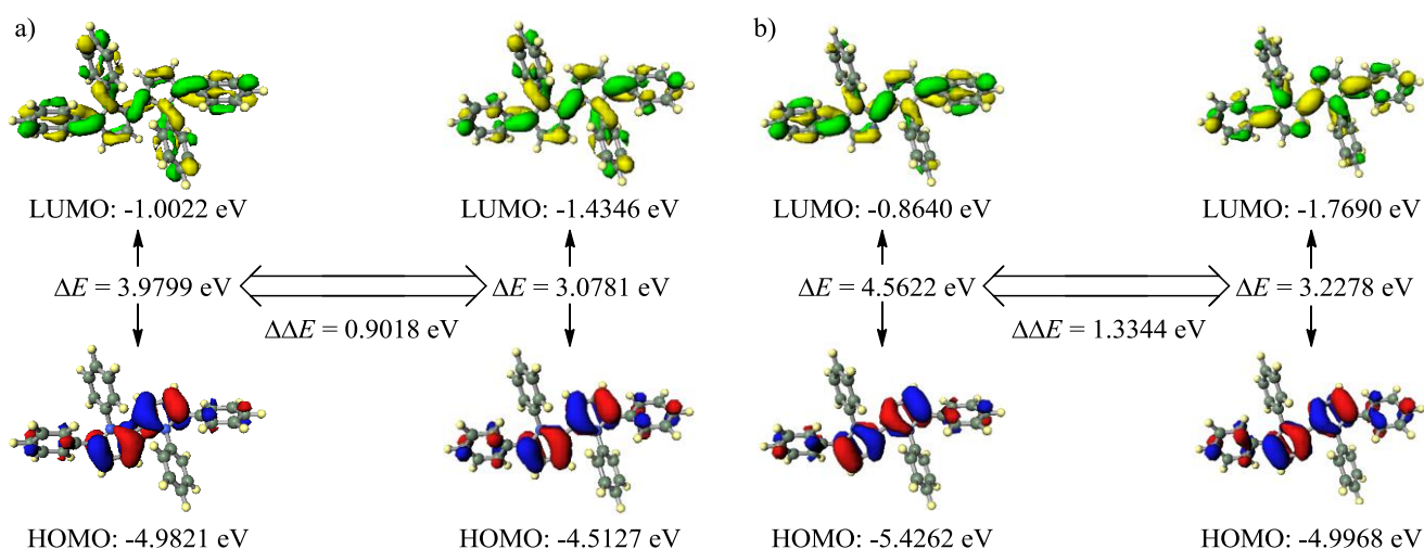
Figure 3. Orbitals and energies of HOMO and LUMO of a) 1 and b) 2, estimated by DFT (left) and TDDFT (nstate=5) (right) calculated for structure optimization at the B3LYP/6-31+G** level
