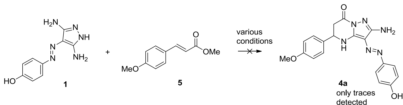
Scheme 2. Conditions: a) 20 mol% ZnCl 2 or HCl, MeOH, reflux/MW; b) 10 - 20 mol% DBU or NaOH, MeOH reflux/MW.
