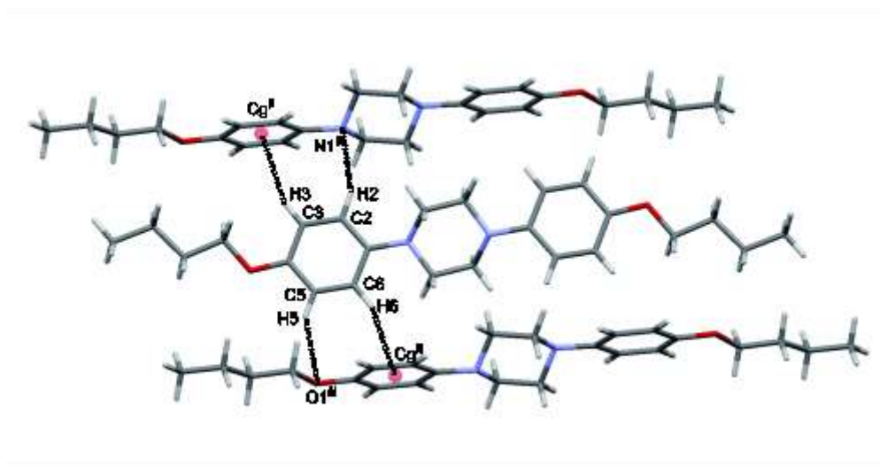
Figure 6. Intermolecular C-H...O, C-H...N, and C-H... \pi interactions of 2 . Cg is the centroid of C1/C2/C3/C4/C5/C6. Symmetry codes: (ii) x, 3/2-y, z-1/2 , (iii) x, 1/2-y, z+1/2
