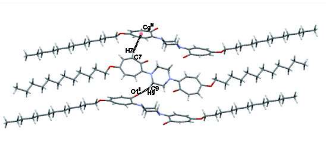
Figure 3. Intermolecular C-H...O and C-H... \pi interactions of 1 . Cg is the centroid of C1/C2/C3/C4/C5/C6/C7 ring. Symmetry codes: (ii) x, 5/2-y, z-1/2 , (iii) x, 3/2-y, z-1/2
