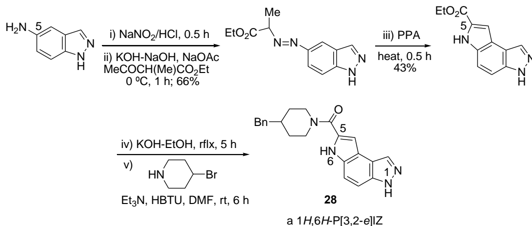
Scheme 17. Fischer/Japp-Klingemann route to a bioactive P[3,2- e ]IZ
