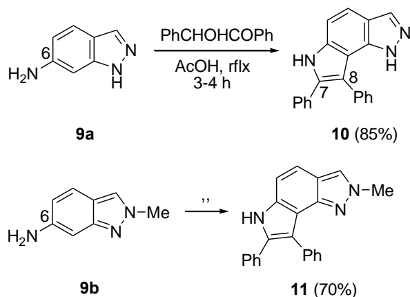
Scheme 7. Heteroannulation of 6-aminoindazoles
