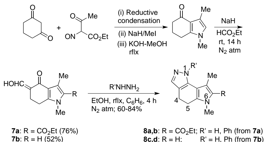
Scheme 6. Further syntheses of 4,5-dihydro-P[2,3-g]IZs from tetrahydroindolones
