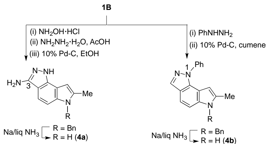
Scheme 3. Synthesis of 3-amino- and 1-phenyl- 2b
