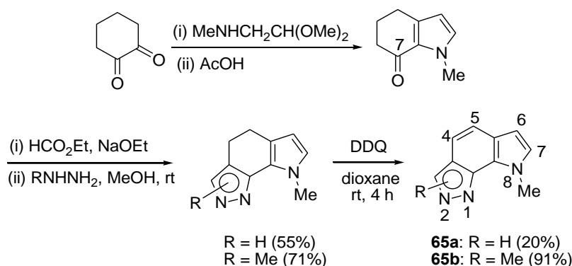
Scheme 33. Synthesis of P[3,2- g ]IZs from N -methyltetrahydroindol-7-one
