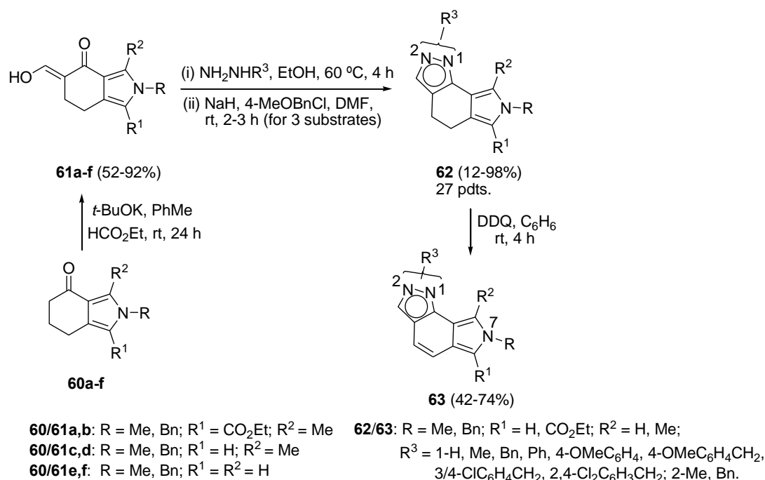
Scheme 30. Synthesis of P[3,4- g ]IZs from tetrahydroisindolones
