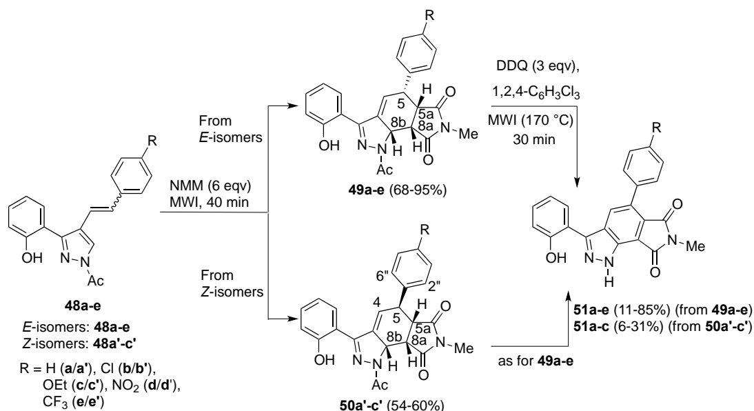
Scheme 27. Cycloaddition of styrylpyrazoles to P[3,4-g]IZs
