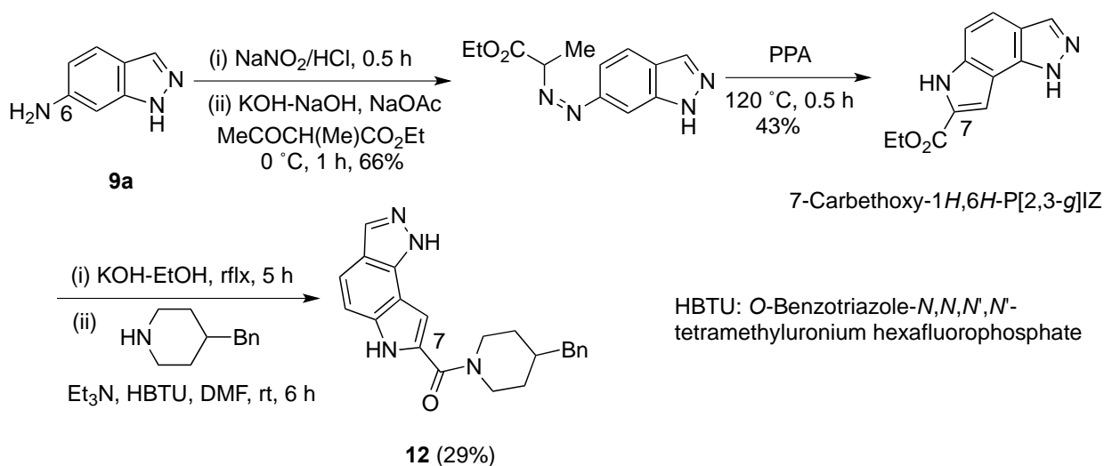
Scheme 8. Fischer/Japp-Klingemann route to a bioactive P[2,3-g]IZ
