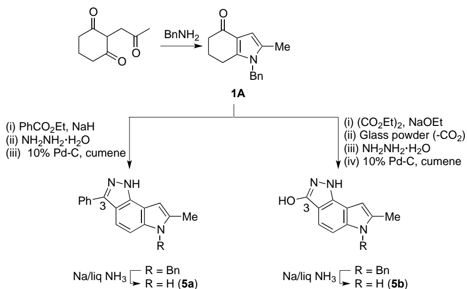
Scheme 4. Synthesis of 3-phenyl- and 3-hydroxy- 2b
