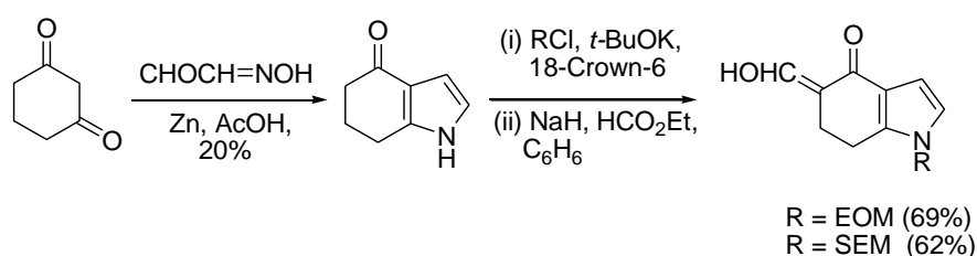
Scheme 10. Synthesis of 5-hydroxymethylenetetrahydroindol-4-ones
