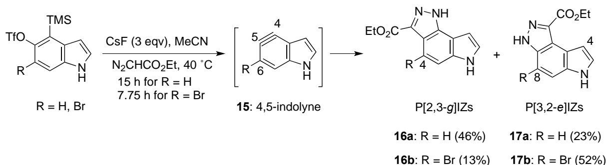
Scheme 11. Synthesis of isomeric PIZs via indolynes
