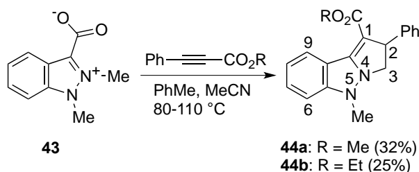
Scheme 25. Synthesis of P[1,2- b ]IZs via cycloaddition of an indazolic betaine
