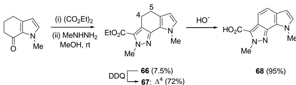
Scheme 34. Similar synthesis of a P[3,2- g ]IZ
