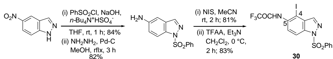
Scheme 20. Synthesis of Sonogashira/Cacchi substrate 30
