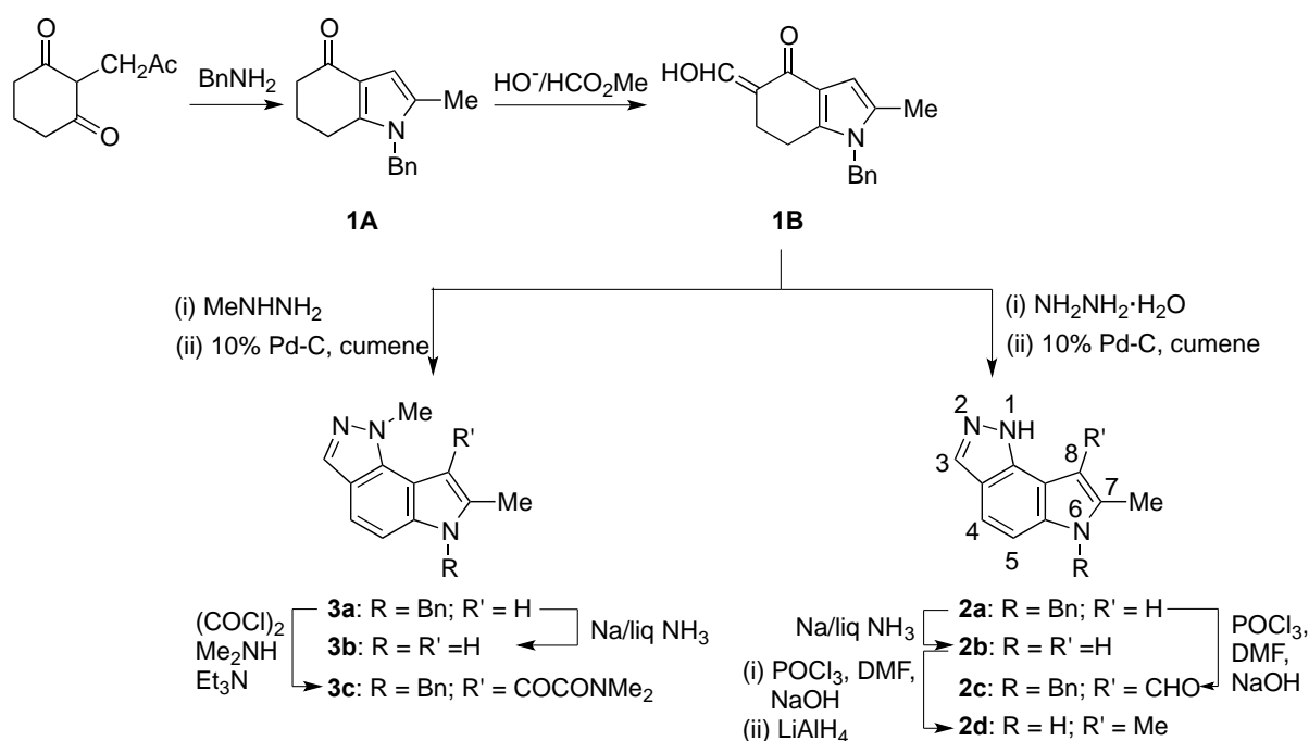
Scheme 1. Synthesis of 7-methyl-P[2,3- g ]IZs
