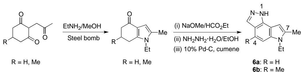
Scheme 5. Synthesis of 6( N )-ethyl analogues of 2b
