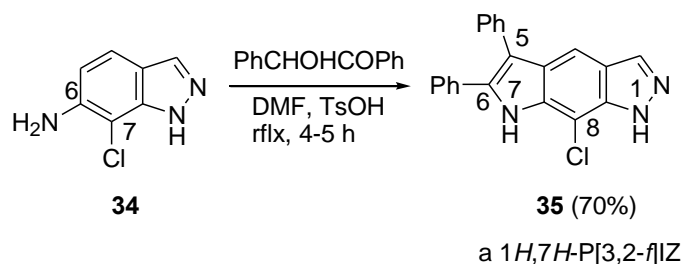
Scheme 21. Only reported synthesis of a P[3,2- f ]IZ
