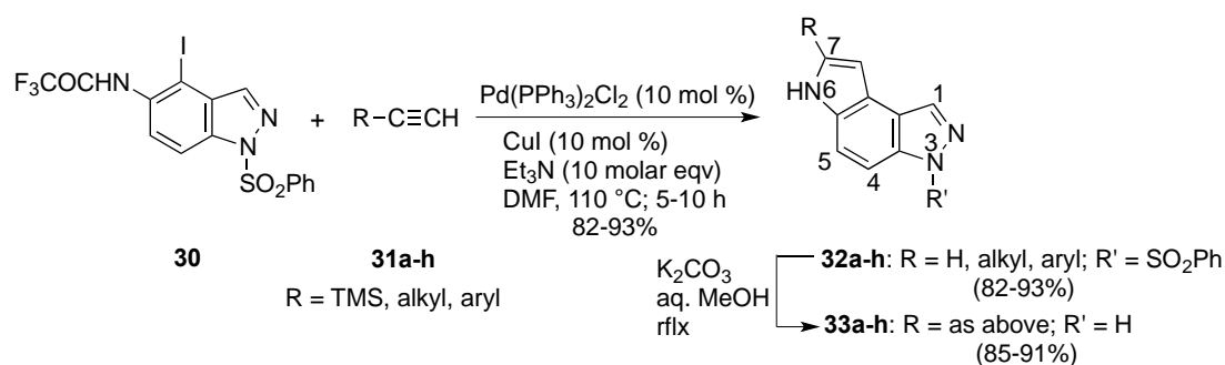
Scheme 19. First general synthesis of 7-substituted P[3,2- e ]IZs
