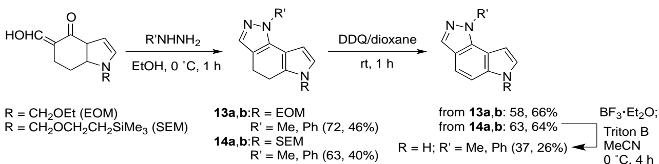
Scheme 9. Synthesis of sGC-inhibitory (dihydro)-P[2,3-g]IZs
