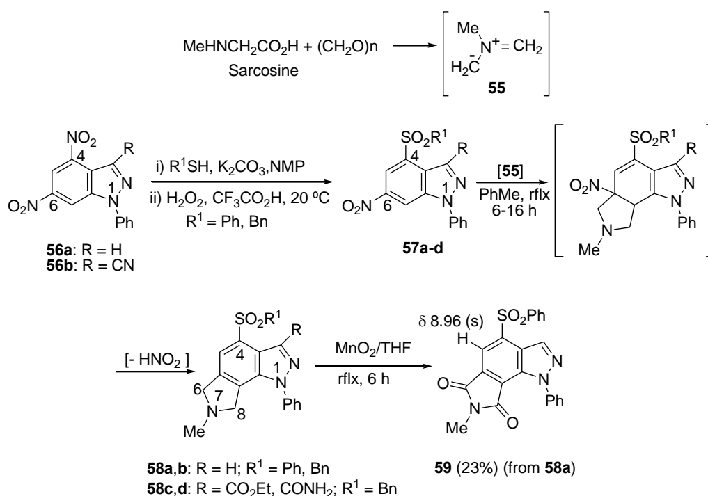
Scheme 29. Azomethine ylide route to P[3,4- g ]IZs
