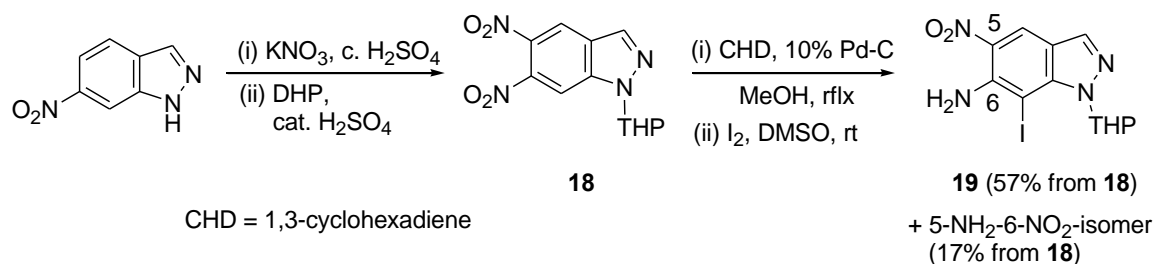
Scheme 12. Synthesis of intermediate for the PIZ 20
