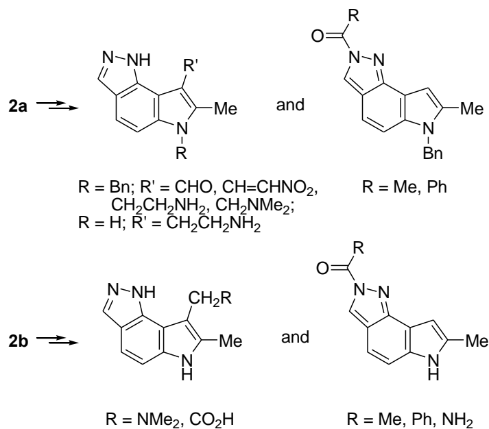
Scheme 2. Synthesis of 1- and 2-substituted analogues of 2a,b
