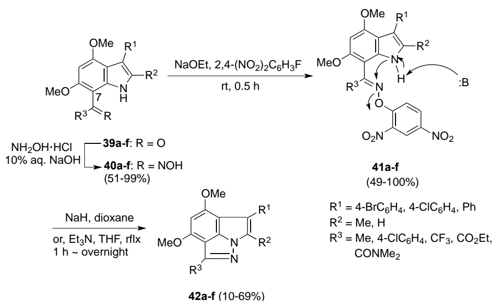
Scheme 24. Only reported synthesis of P[3,2,1- hi ]IZs
