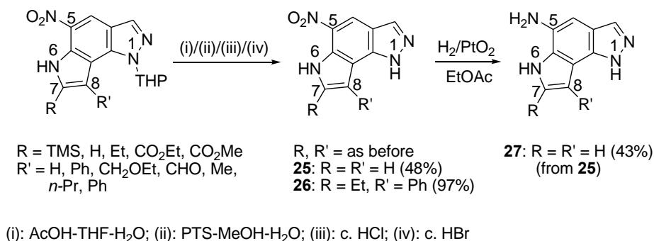
Scheme 16. Transformations to Pim kinase-inhibitory P[2,3- g ]IZs
