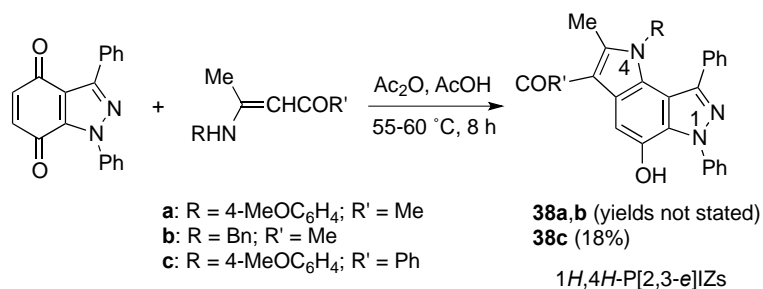
Scheme 23. Further synthesis of P[2,3- e ]IZs using enaminoketones
