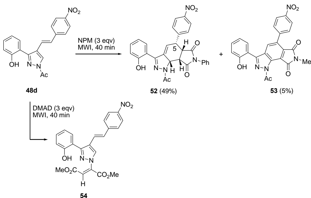
Scheme 28. Similar synthesis of P[3,4-g]IZs
