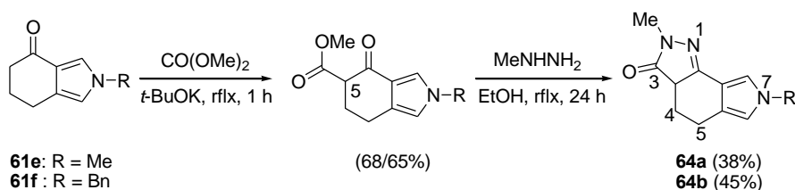
Scheme 32. Similar synthesis of P[3,4- g ]IZ-3-ones
