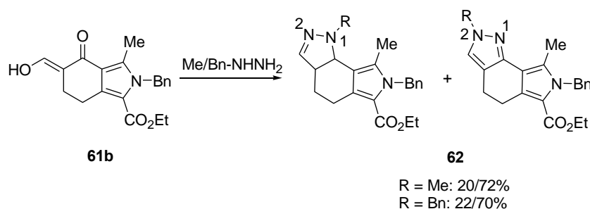
Scheme 31. Similar synthesis of other P[3,4- g ]IZs
