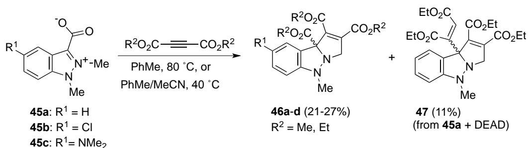
Scheme 26. Analogous synthesis of further P[1,2- b ]IZs
