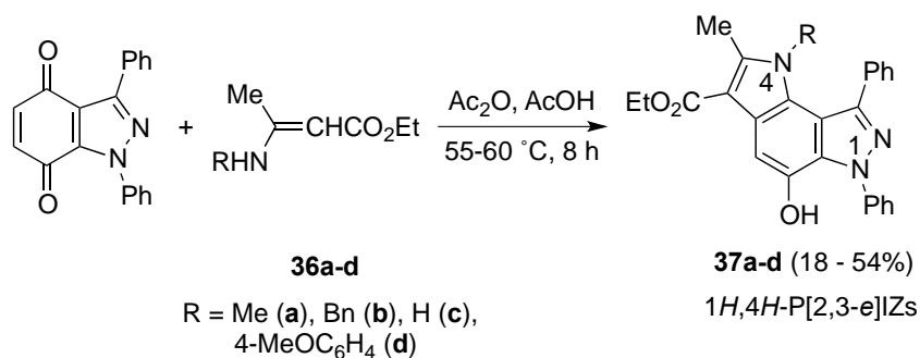
Scheme 22. First synthesis of P[2,3- e ]IZs using Nenitzescu reaction
