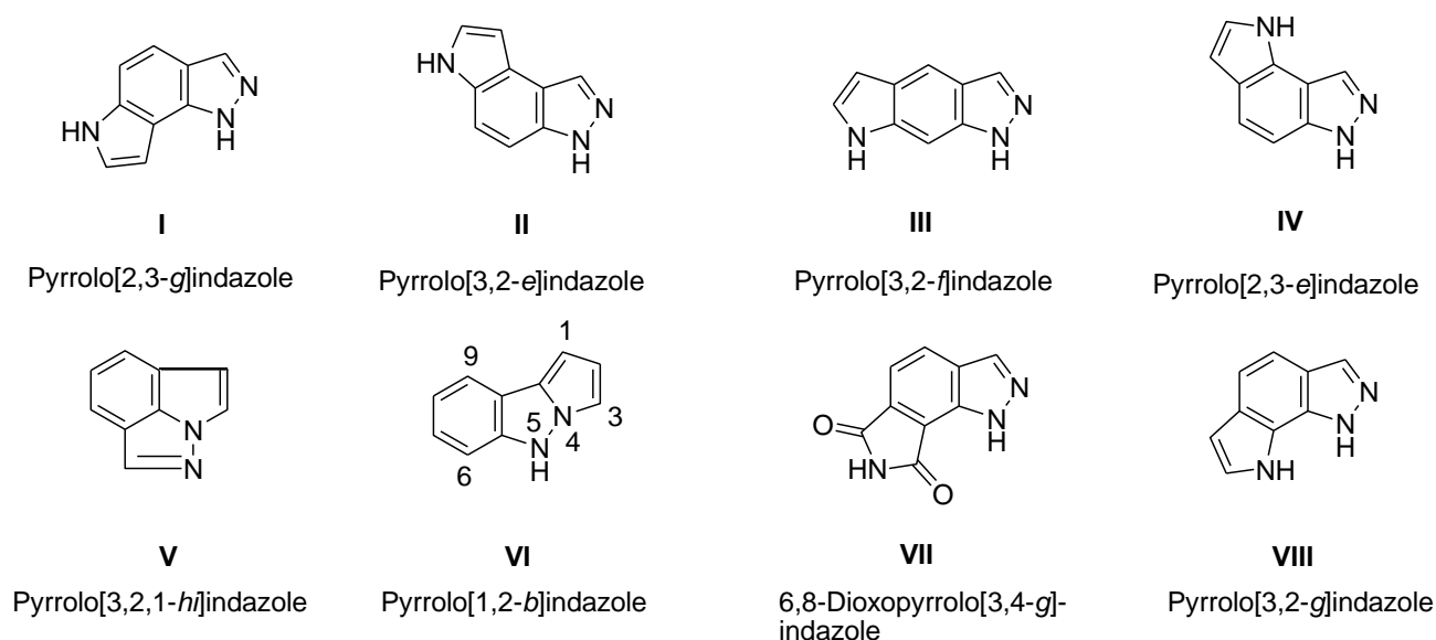
Figure 1. Isomeric pyrroloindazoles reported till date
