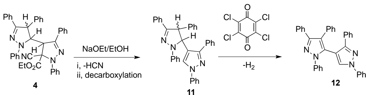
Scheme 3. Synthesis of the bipyrazoles 11 and 12
