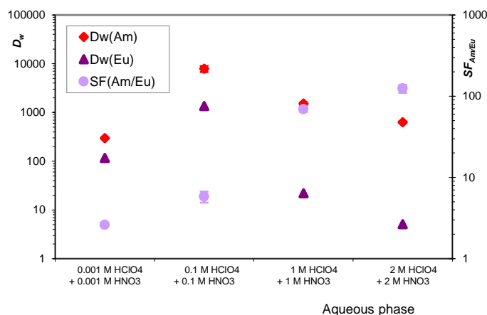
Figure 6. Extraction of Am(III) and Eu(III) by CyMe 4 -BTPPhen-functionalized SiO 2 gel 8 as a function of HClO 4 /HNO 3 concentration. Mass of sorbent: approximately 15 mg, phase volume: 0.6 mL, V/m ratio: ~ 40 mL g -1
