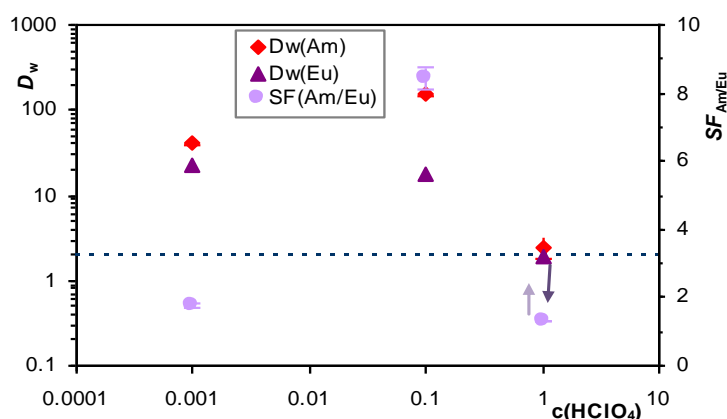
Figure 5. Extraction of Am(III) and Eu(III) by CyMe 4 -BTPPhen-functionalized SiO 2 -coated MNPs 4 as a function of HClO 4 concentration. Mass of sorbent: approximately 18 mg, phase volume: 0.6 mL, V/m ratio: ~ 33 mL g -1
