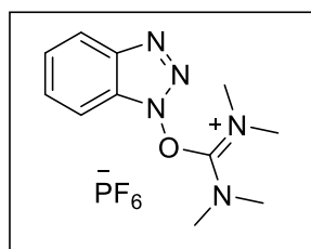
Figure 1. Structure of O -benzotriazol-1-yl)- N,N,N',N' -tetramethyluronium hexafluorophosphate (HBTU)
