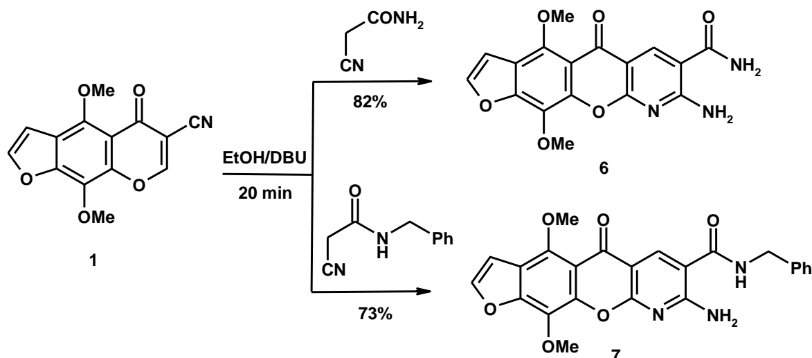
Scheme 3. Formation of furo[3',2':6,7]chromeno[2,3- b ]pyridines 6 and 7
