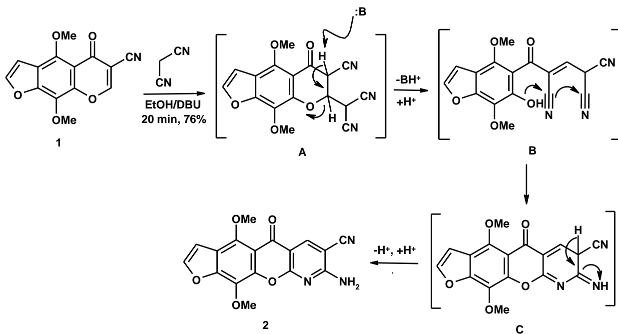
Scheme 1. Formation of furo[3'',2'':6,7]chromeno[2,3- b ]pyridine-7-carbonitrile 2
