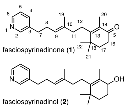
Figure 1. Chemical structures of fasciospyrinadinone ( 1 ) and fasciospyrinadinol ( 2 )
