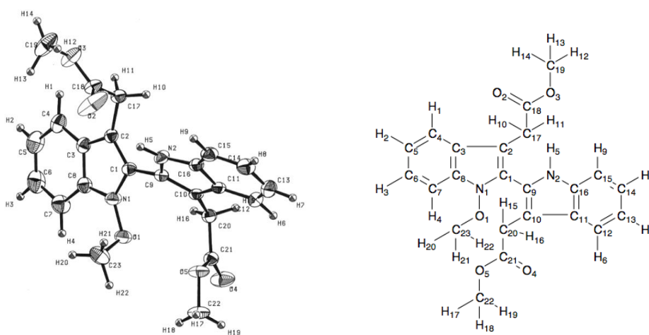
Figure 2. ORTEP drawing and numbering of 53
