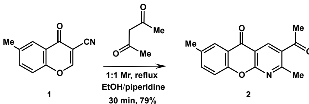
Scheme 1. Synthesis of 3-acetyl-2,7-dimethyl-5 H -chromeno[2,3- b ]pyridin-5-one ( 2 )
