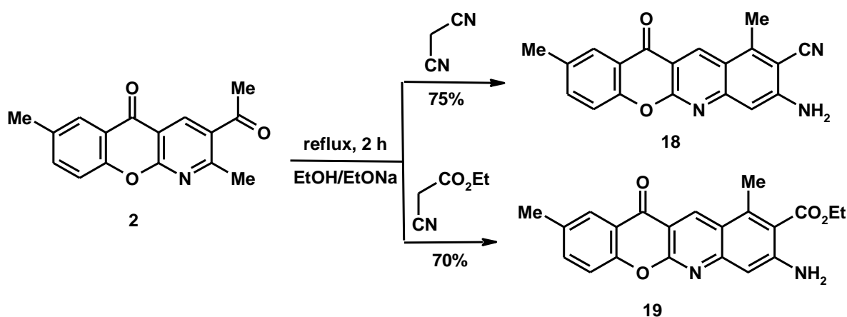
Scheme 6. Formation of chromeno[2,3- b ]quinoline derivatives 18 and 19
