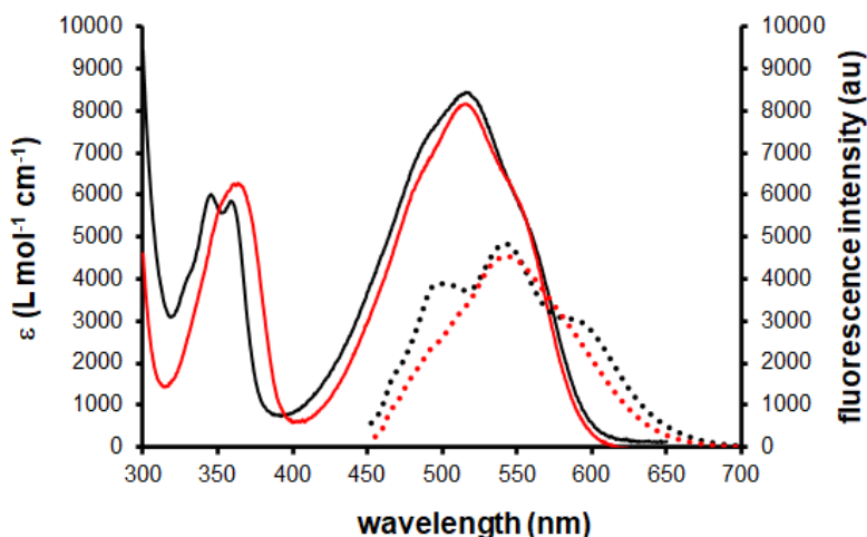
Figure 2. UV-Vis (solid lines) and fluorescence spectra (dashed lines) of 1a upon excitation at 410 nm in MeCN ( c = 1 \times 10^{-4} M, black) and MeOH ( c = 1 \times 10^{-4} M, red) at 25 °C
