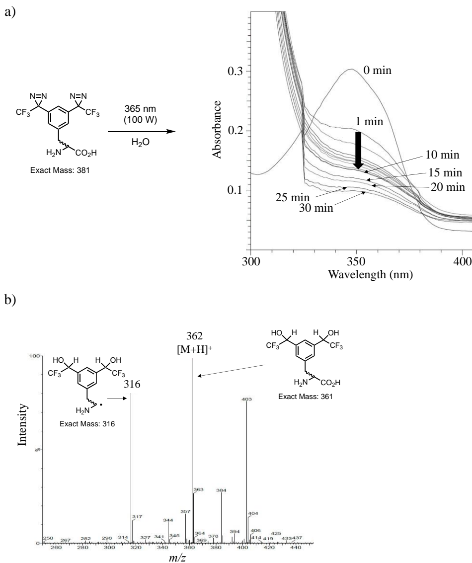
Figure 2. a) Photolysis of bis-diaziriny-Phe 13 in H 2 O (1 mM) under black light (100 W). UV spectra of the photolysis were recorded every minute for 10 min. b) ESI-MS analysis of a mixture of products after photoirradiation of compound 13 for 10 minutes.
