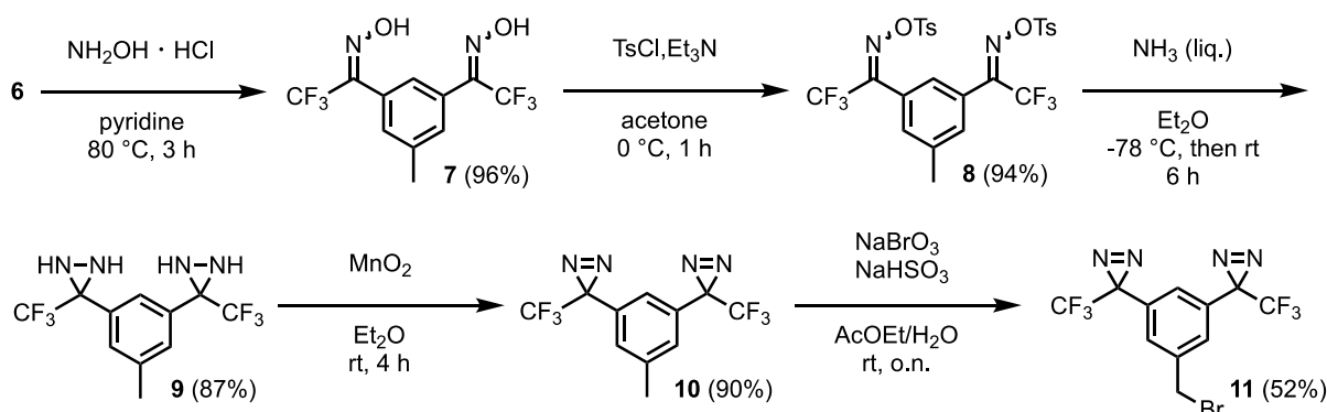
Scheme 2. Preparation of 3,5-bis-diazirinyl-benzyl bromide 11
