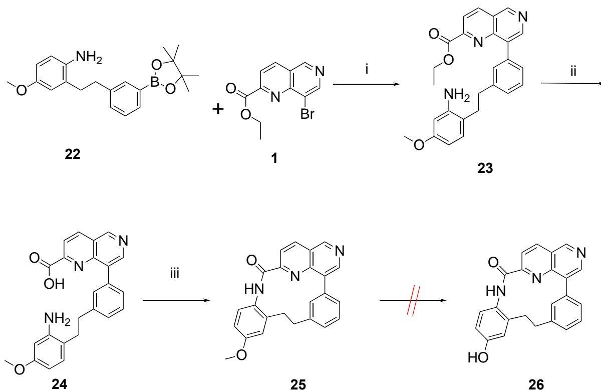
Scheme 4. Reagents and conditions: i. \text{Pd}(\text{PPh}_3)_2\text{Cl}_2 , KF, dioxane, water (66%), ii. LiOH, THF, water (71%), iii. CDI, DCM, pyridine (26%).
