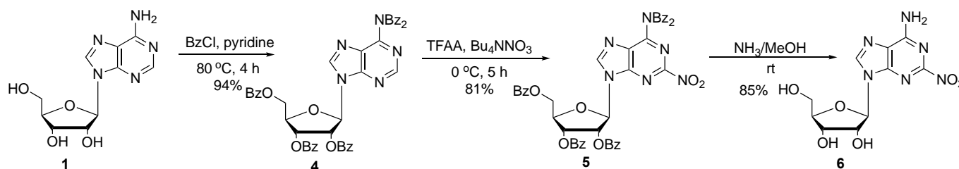
Scheme 4. The synthetic route of 2-nitroadenosine ( 6 )
