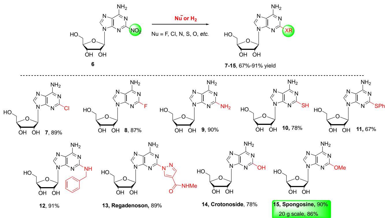
Scheme 5. The synthesis of 2-substituted adenosines
